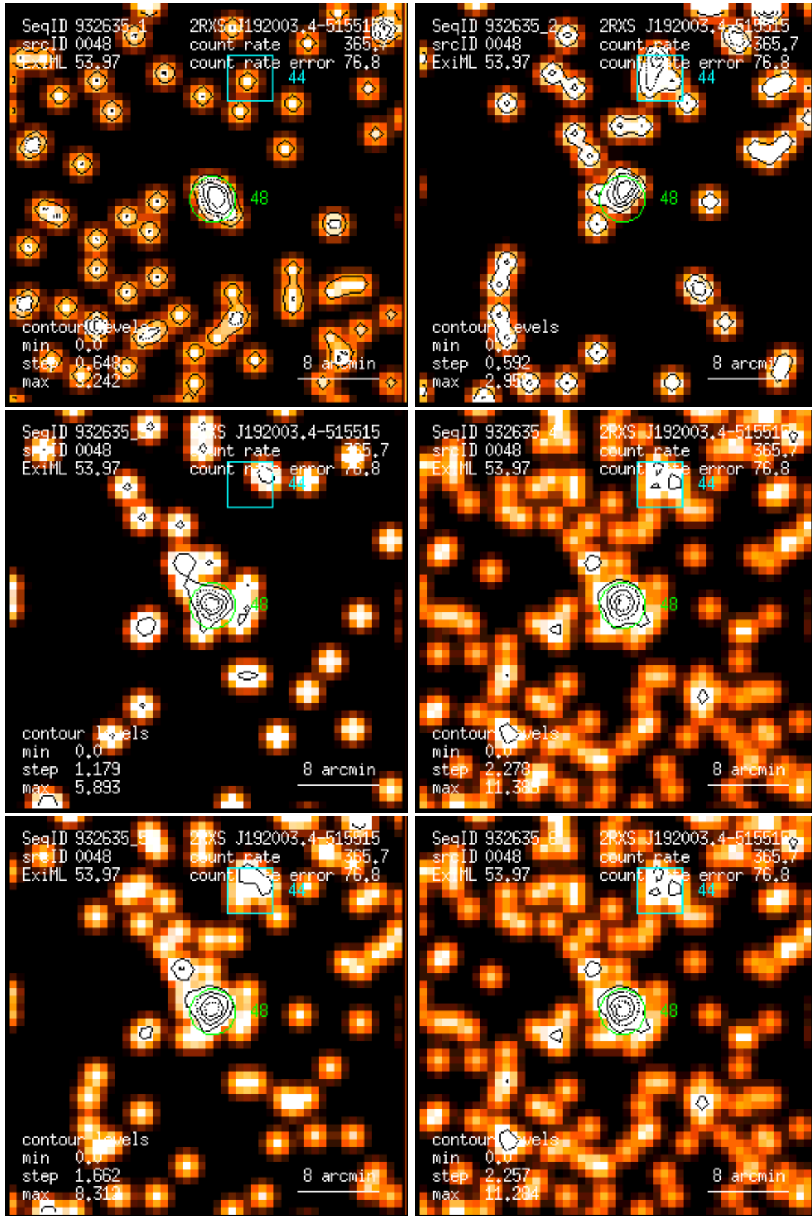
Figure 48: RASS 932635: detection 0048: band rate images, Gaussian filter: (1) PSPC channels 11 – 41, (2) 52 – 90, (3) 91 – 201, (4) 11 – 235, (5) 52 – 201, (6) 11 – 201. Broad band rates in counts/ks. Band rate contour levels in counts/ks/arcmin 2 .
