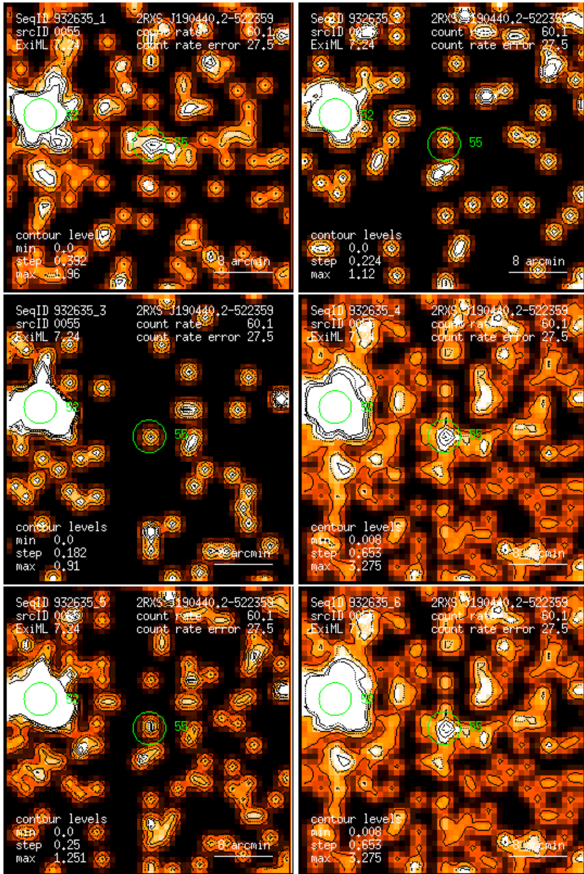
Figure 55: RASS 932635: detection 0055: band rate images, Gaussian filter: (1) PSPC channels 11 – 41, (2) 52 – 90, (3) 91 – 201, (4) 11 – 235, (5) 52 – 201, (6) 11 – 201. Broad band rates in counts/ks. Band rate contour levels in counts/ks/arcmin 2 .
