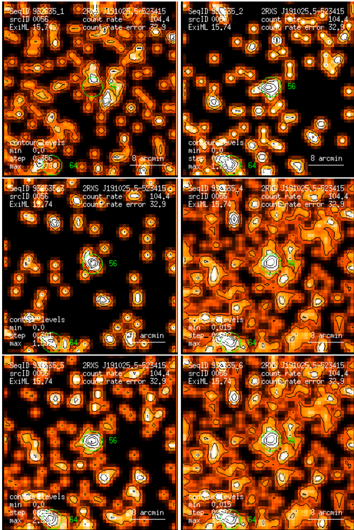
Figure 56: RASS 932635: detection 0056: band rate images, Gaussian filter: (1) PSPC channels 11 – 41, (2) 52 – 90, (3) 91 – 201, (4) 11 – 235, (5) 52 – 201, (6) 11 – 201. Broad band rates in counts/ks. Band rate contour levels in counts/ks/arcmin 2 .
