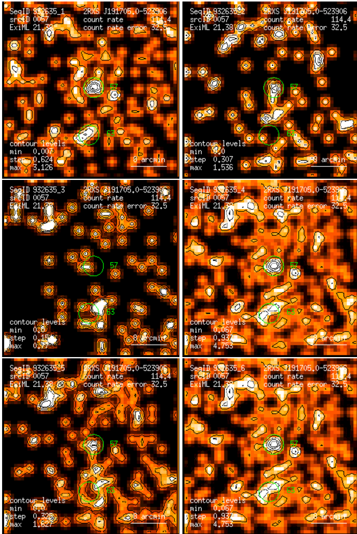
Figure 57: RASS 932635: detection 0057: band rate images, Gaussian filter: (1) PSPC channels 11 – 41, (2) 52 – 90, (3) 91 – 201, (4) 11 – 235, (5) 52 – 201, (6) 11 – 201. Broad band rates in counts/ks. Band rate contour levels in counts/ks/arcmin 2 .
