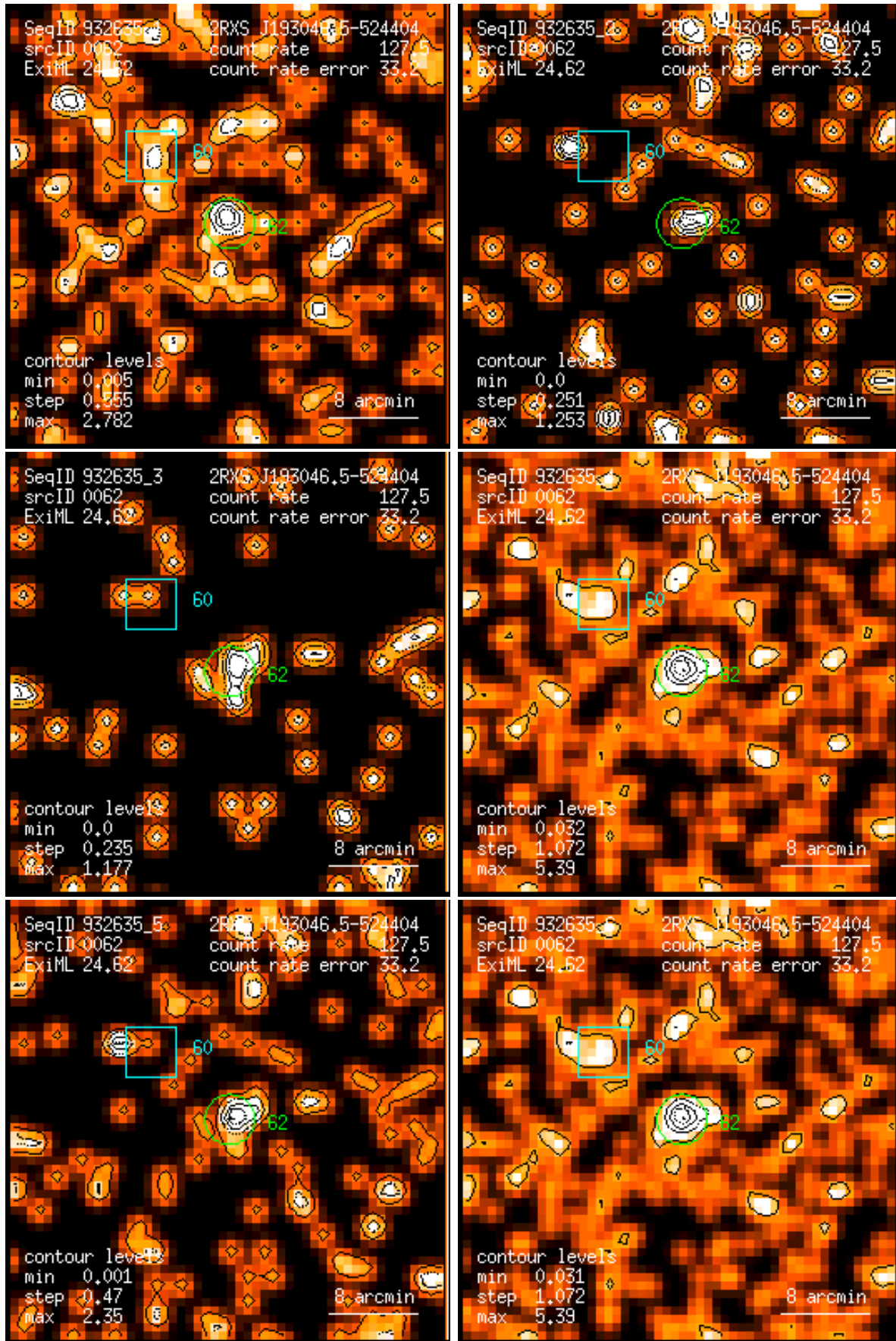
Figure 62: RASS 932635: detection 0062: band rate images, Gaussian filter: (1) PSPC channels 11 – 41, (2) 52 – 90, (3) 91 – 201, (4) 11 – 235, (5) 52 – 201, (6) 11 – 201. Broad band rates in counts/ks. Band rate contour levels in counts/ks/arcmin 2 .
