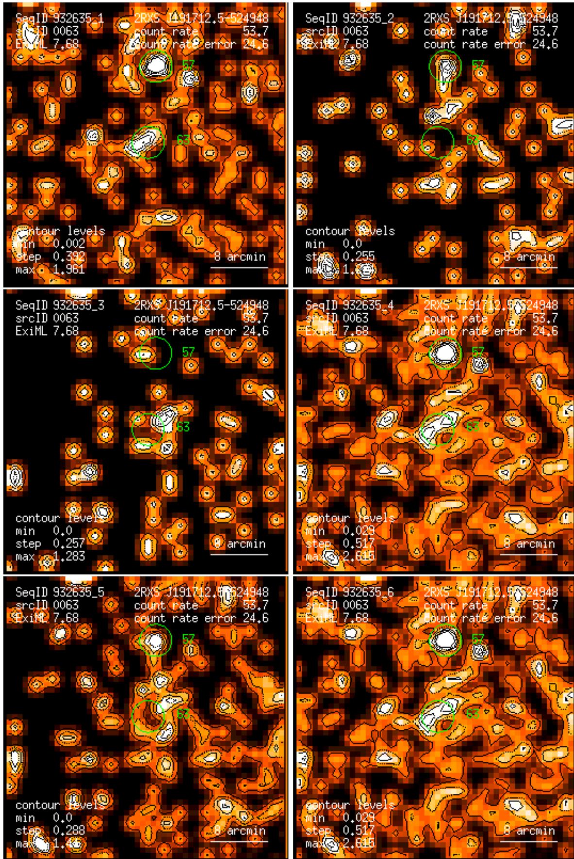
Figure 63: RASS 932635: detection 0063: band rate images, Gaussian filter: (1) PSPC channels 11 – 41, (2) 52 – 90, (3) 91 – 201, (4) 11 – 235, (5) 52 – 201, (6) 11 – 201. Broad band rates in counts/ks. Band rate contour levels in counts/ks/arcmin 2 .
