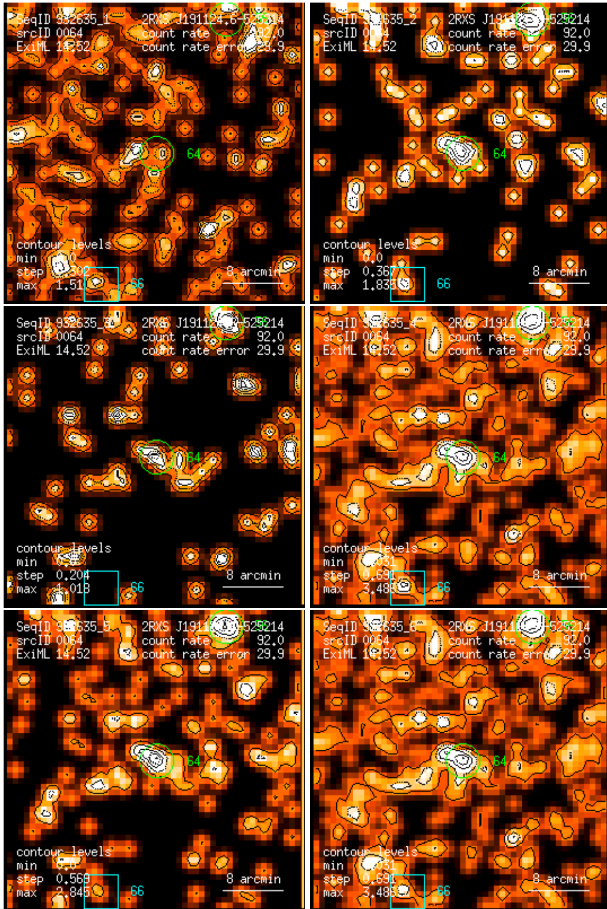
Figure 64: RASS 932635: detection 0064: band rate images, Gaussian filter: (1) PSPC channels 11 – 41, (2) 52 – 90, (3) 91 – 201, (4) 11 – 235, (5) 52 – 201, (6) 11 – 201. Broad band rates in counts/ks. Band rate contour levels in counts/ks/arcmin 2 .
