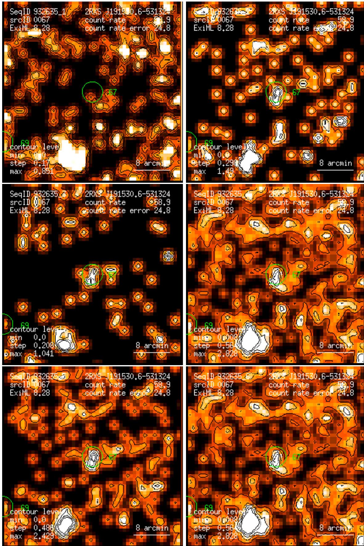
Figure 67: RASS 932635: detection 0067: band rate images, Gaussian filter: (1) PSPC channels 11 – 41, (2) 52 – 90, (3) 91 – 201, (4) 11 – 235, (5) 52 – 201, (6) 11 – 201. Broad band rates in counts/ks. Band rate contour levels in counts/ks/arcmin 2 .
