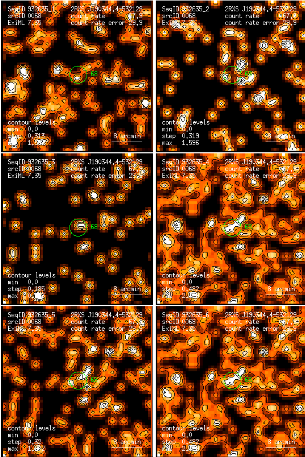
Figure 68: RASS 932635: detection 0068: band rate images, Gaussian filter: (1) PSPC channels 11 – 41, (2) 52 – 90, (3) 91 – 201, (4) 11 – 235, (5) 52 – 201, (6) 11 – 201. Broad band rates in counts/ks. Band rate contour levels in counts/ks/arcmin 2 .
