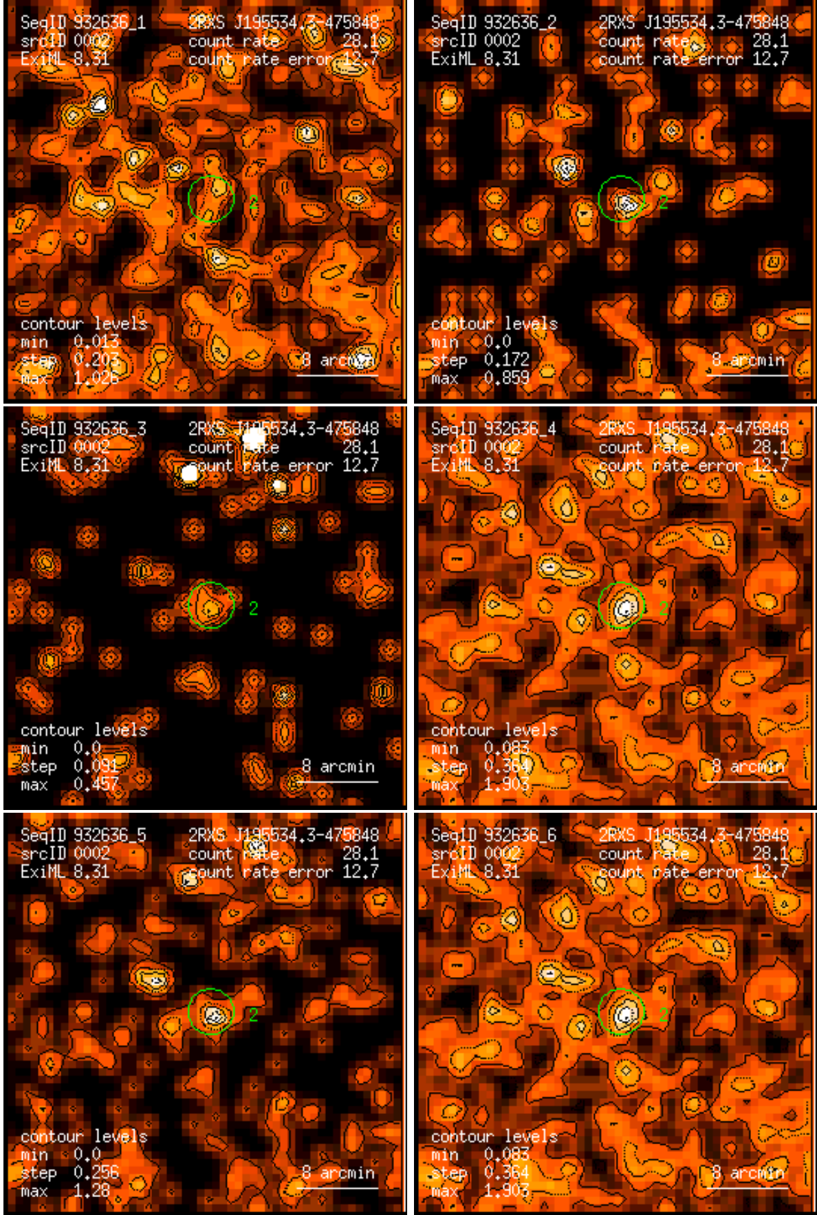
Figure 2: RASS 932636: detection 0002: band rate images, Gaussian filter: (1) PSPC channels 11 – 41, (2) 52 – 90, (3) 91 – 201, (4) 11 – 235, (5) 52 – 201, (6) 11 – 201. Broad band rates in counts/ks. Band rate contour levels in counts/ks/arcmin 2 .
