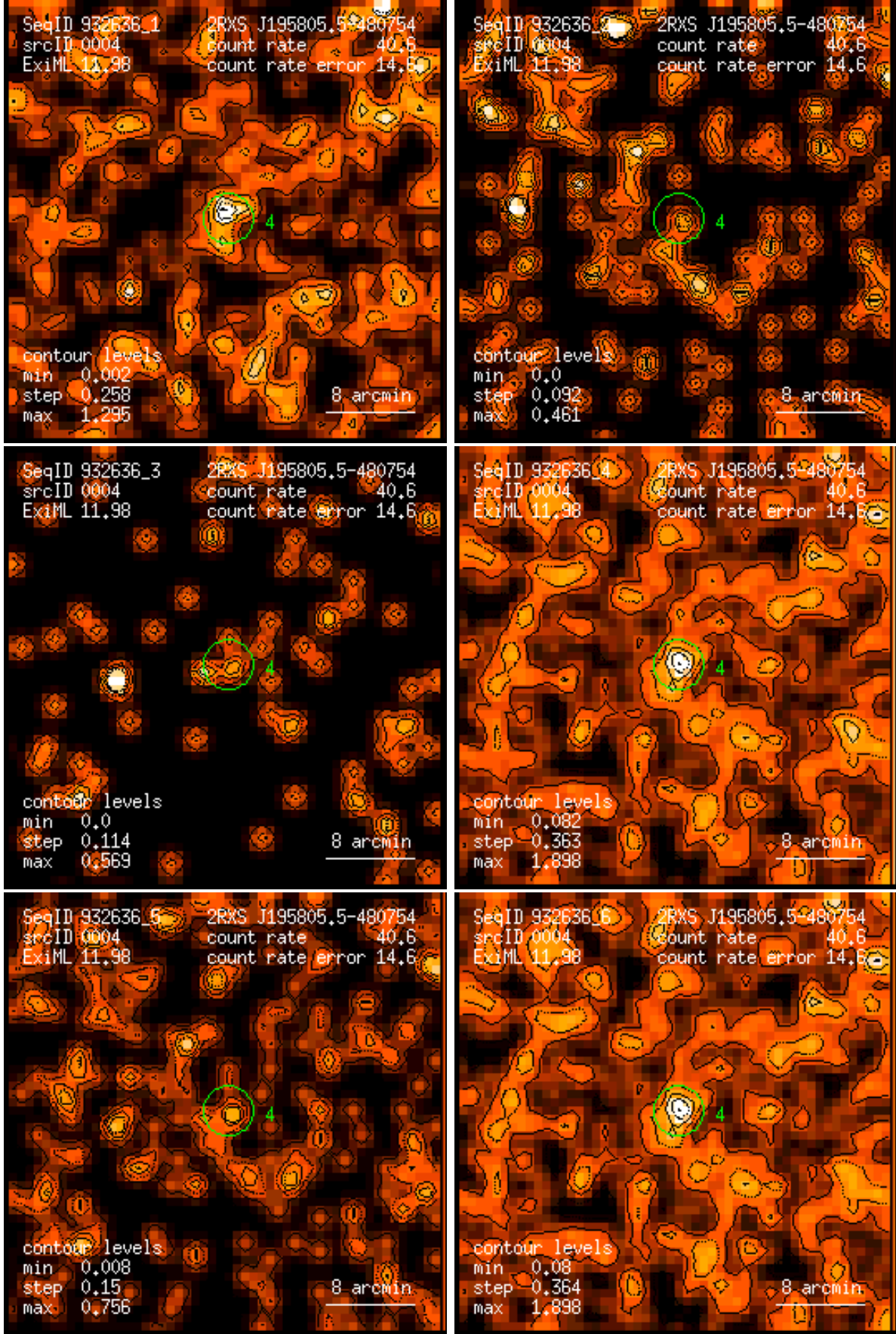
Figure 4: RASS 932636: detection 0004: band rate images, Gaussian filter: (1) PSPC channels 11 – 41, (2) 52 – 90, (3) 91 – 201, (4) 11 – 235, (5) 52 – 201, (6) 11 – 201. Broad band rates in counts/ks. Band rate contour levels in counts/ks/arcmin 2 .
