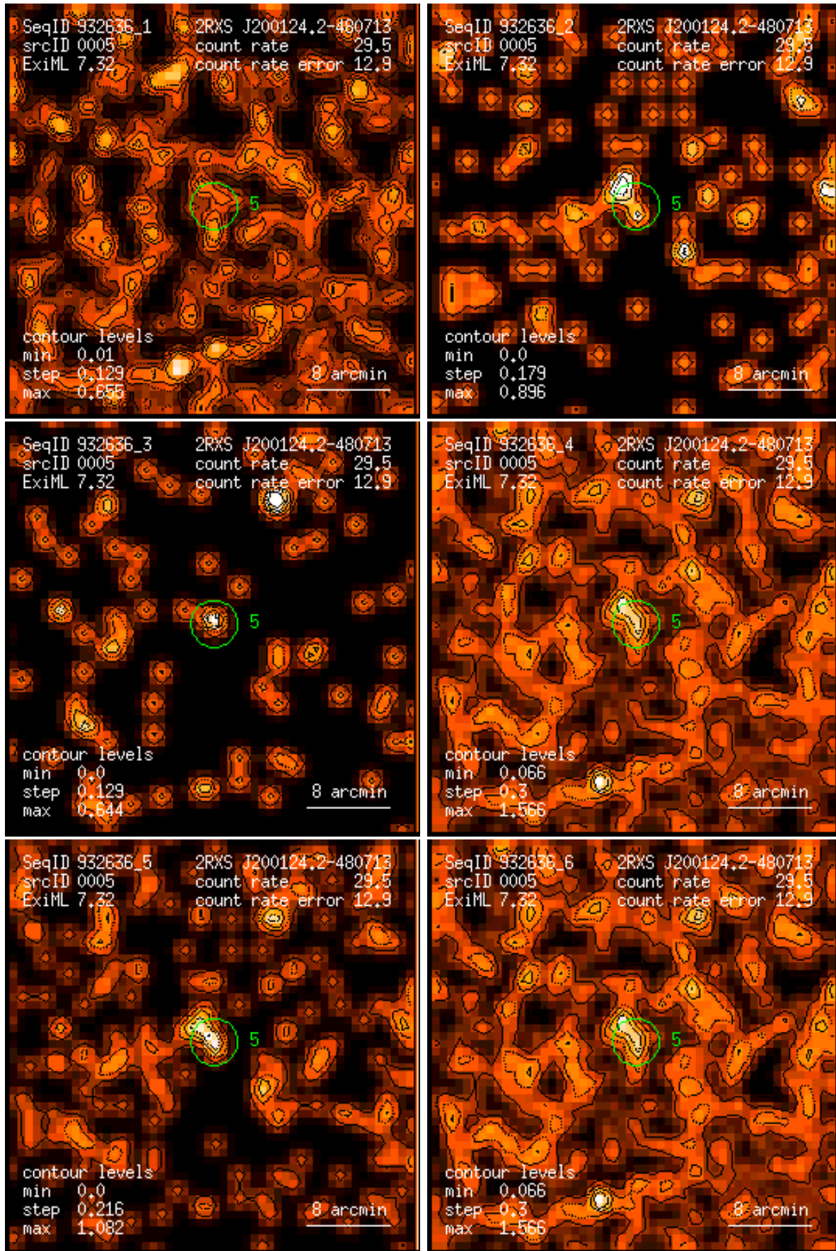
Figure 5: RASS 932636: detection 0005: band rate images, Gaussian filter: (1) PSPC channels 11 – 41, (2) 52 – 90, (3) 91 – 201, (4) 11 – 235, (5) 52 – 201, (6) 11 – 201. Broad band rates in counts/ks. Band rate contour levels in counts/ks/arcmin 2 .
