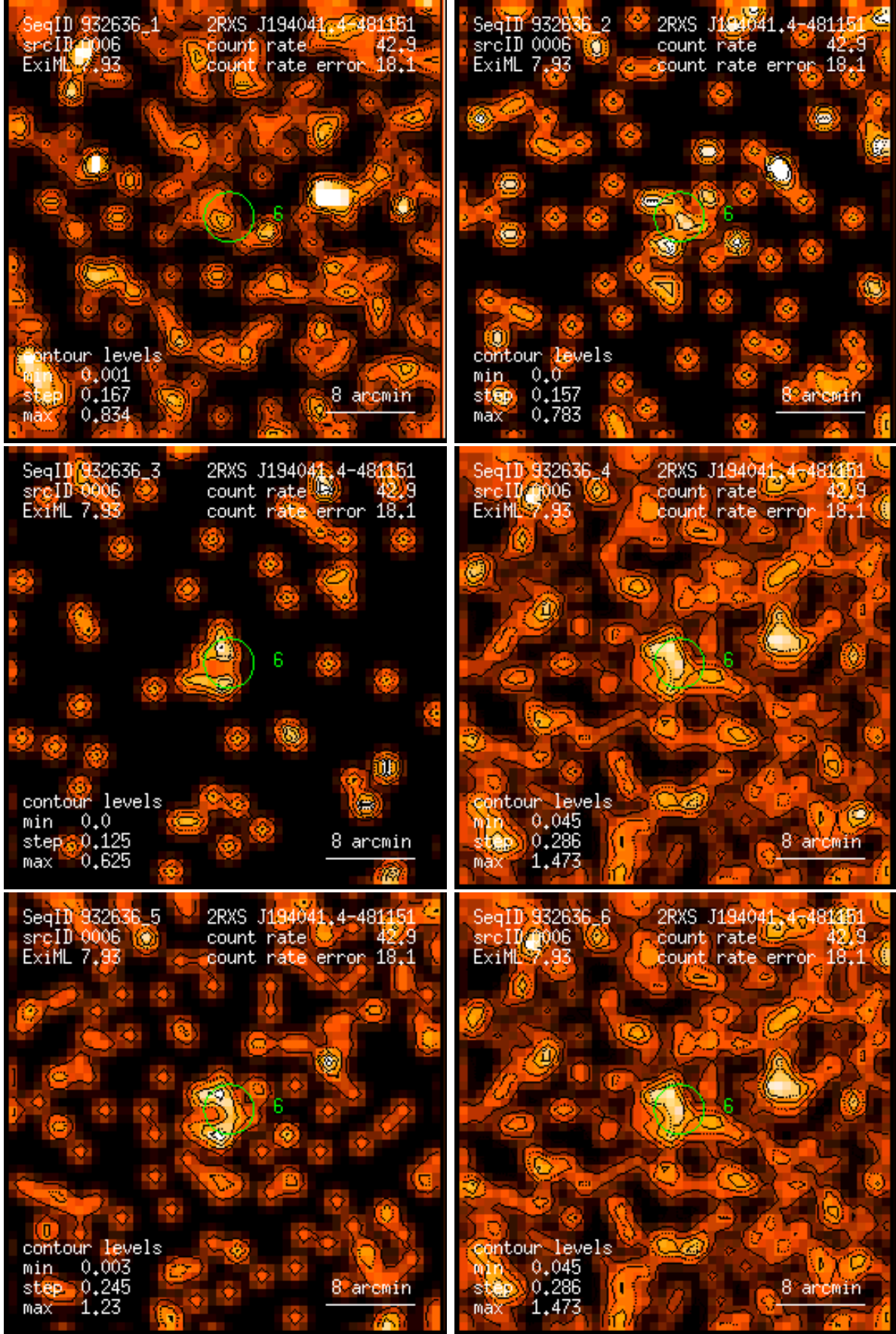
Figure 6: RASS 932636: detection 0006: band rate images, Gaussian filter: (1) PSPC channels 11 – 41, (2) 52 – 90, (3) 91 – 201, (4) 11 – 235, (5) 52 – 201, (6) 11 – 201. Broad band rates in counts/ks. Band rate contour levels in counts/ks/arcmin 2 .
