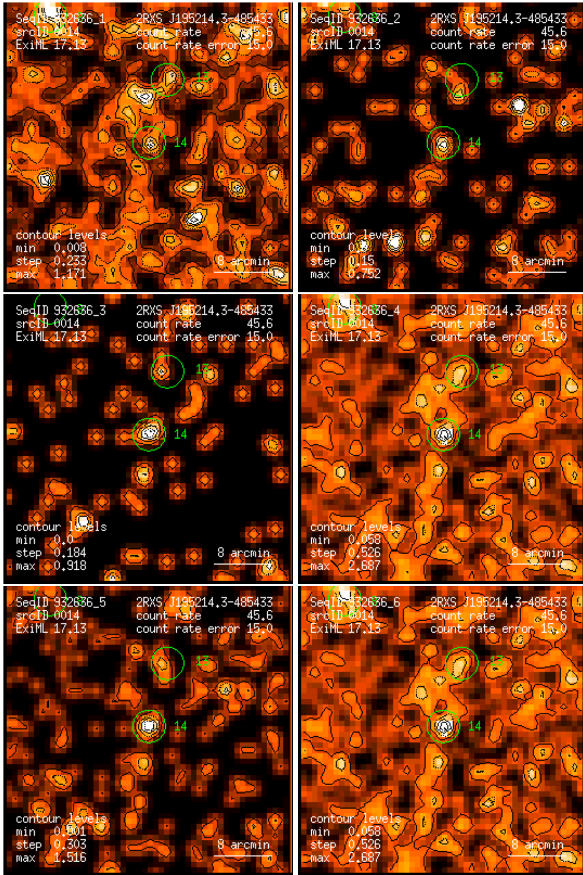
Figure 14: RASS 932636: detection 0014: band rate images, Gaussian filter: (1) PSPC channels 11 – 41, (2) 52 – 90, (3) 91 – 201, (4) 11 – 235, (5) 52 – 201, (6) 11 – 201. Broad band rates in counts/ks. Band rate contour levels in counts/ks/arcmin 2 .
