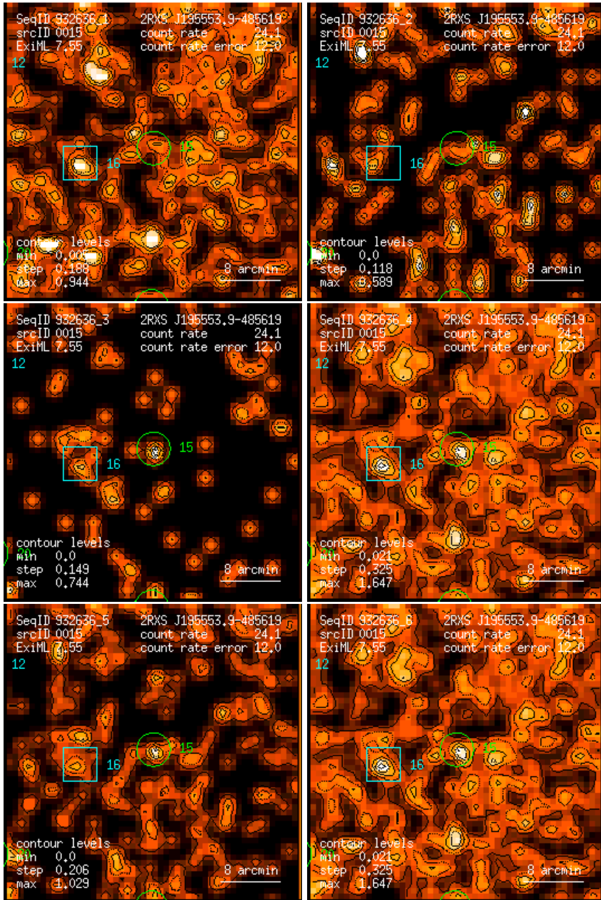
Figure 15: RASS 932636: detection 0015: band rate images, Gaussian filter: (1) PSPC channels 11 – 41, (2) 52 – 90, (3) 91 – 201, (4) 11 – 235, (5) 52 – 201, (6) 11 – 201. Broad band rates in counts/ks. Band rate contour levels in counts/ks/arcmin 2 .
