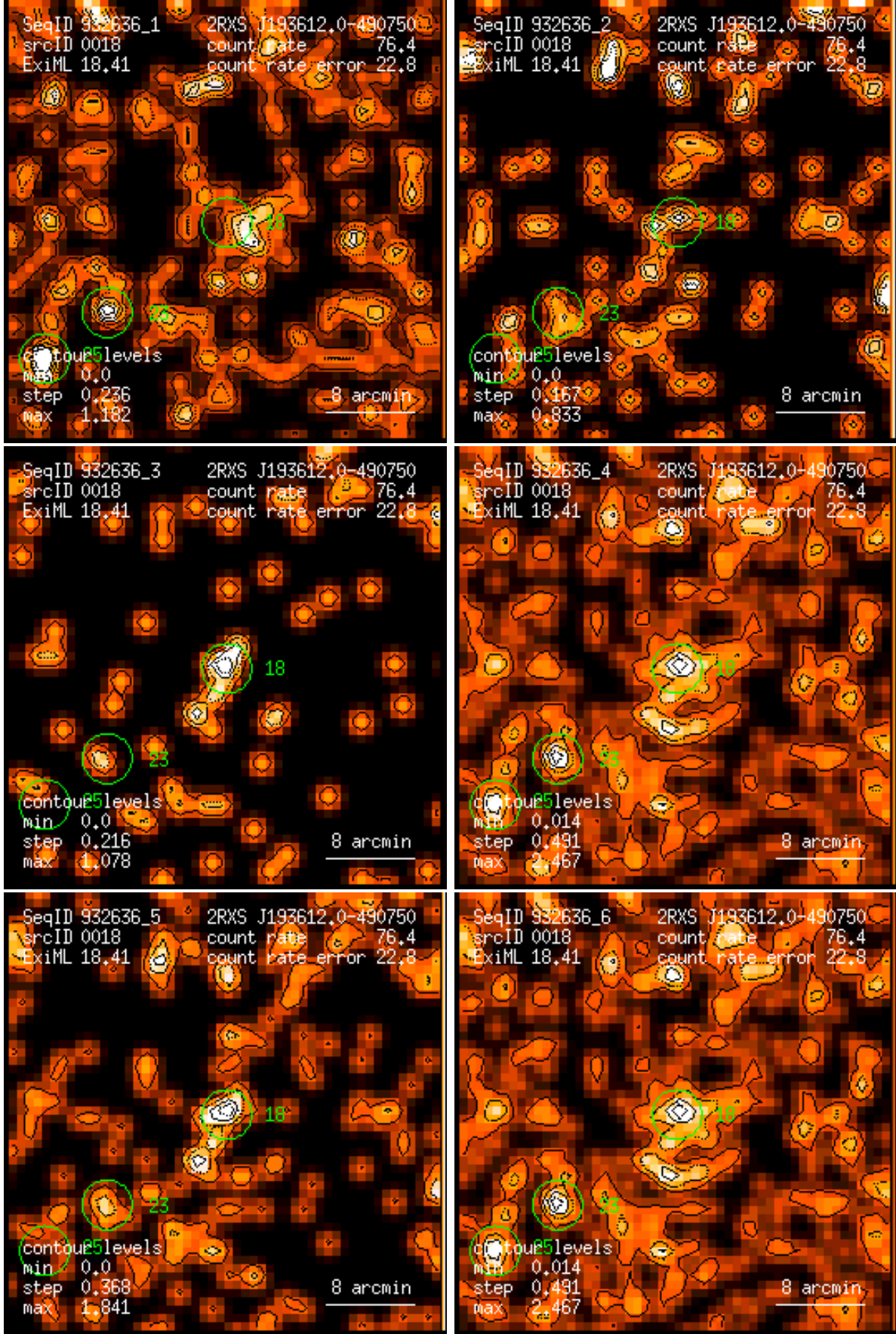
Figure 18: RASS 932636: detection 0018: band rate images, Gaussian filter: (1) PSPC channels 11 – 41, (2) 52 – 90, (3) 91 – 201, (4) 11 – 235, (5) 52 – 201, (6) 11 – 201. Broad band rates in counts/ks. Band rate contour levels in counts/ks/arcmin 2 .
