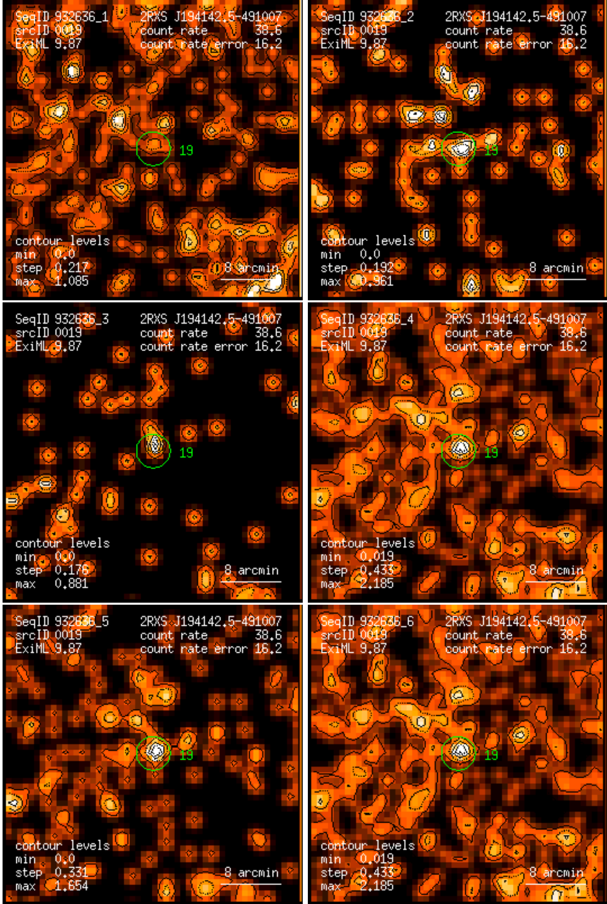
Figure 19: RASS 932636: detection 0019: band rate images, Gaussian filter: (1) PSPC channels 11 – 41, (2) 52 – 90, (3) 91 – 201, (4) 11 – 235, (5) 52 – 201, (6) 11 – 201. Broad band rates in counts/ks. Band rate contour levels in counts/ks/arcmin 2 .
