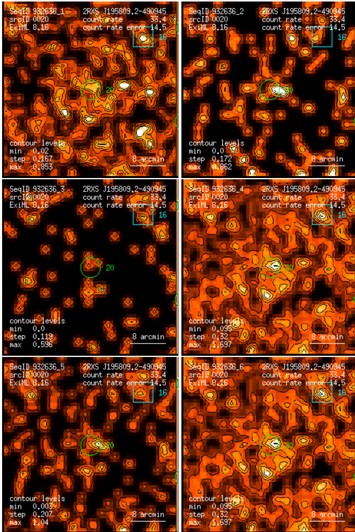
Figure 20: RASS 932636: detection 0020: band rate images, Gaussian filter: (1) PSPC channels 11 – 41, (2) 52 – 90, (3) 91 – 201, (4) 11 – 235, (5) 52 – 201, (6) 11 – 201. Broad band rates in counts/ks. Band rate contour levels in counts/ks/arcmin 2 .
