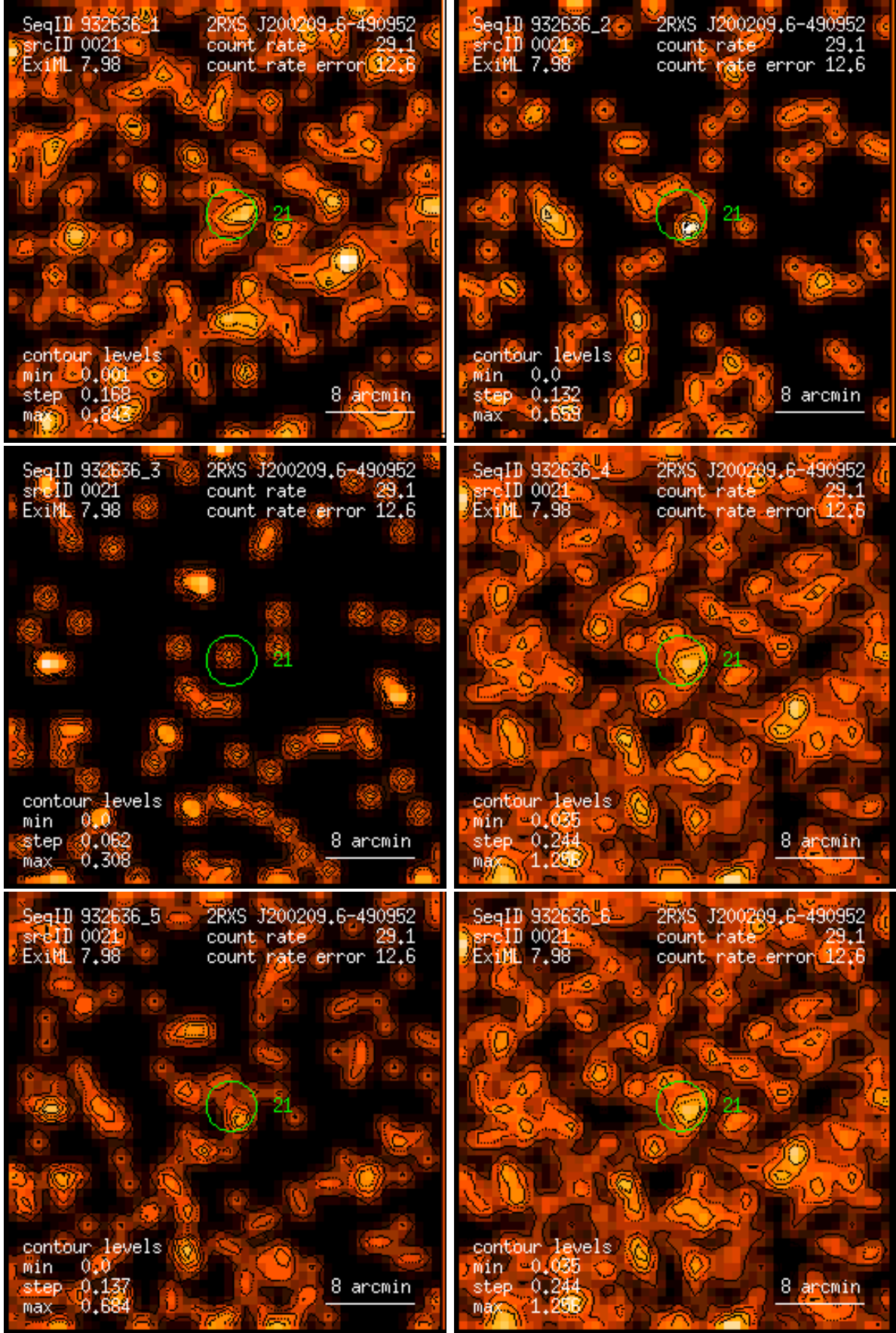
Figure 21: RASS 932636: detection 0021: band rate images, Gaussian filter: (1) PSPC channels 11 – 41, (2) 52 – 90, (3) 91 – 201, (4) 11 – 235, (5) 52 – 201, (6) 11 – 201. Broad band rates in counts/ks. Band rate contour levels in counts/ks/arcmin 2 .
