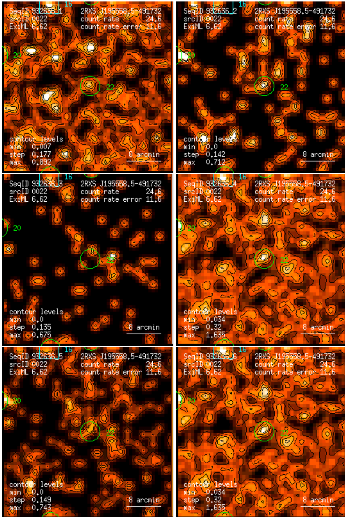
Figure 22: RASS 932636: detection 0022: band rate images, Gaussian filter: (1) PSPC channels 11 – 41, (2) 52 – 90, (3) 91 – 201, (4) 11 – 235, (5) 52 – 201, (6) 11 – 201. Broad band rates in counts/ks. Band rate contour levels in counts/ks/arcmin 2 .
