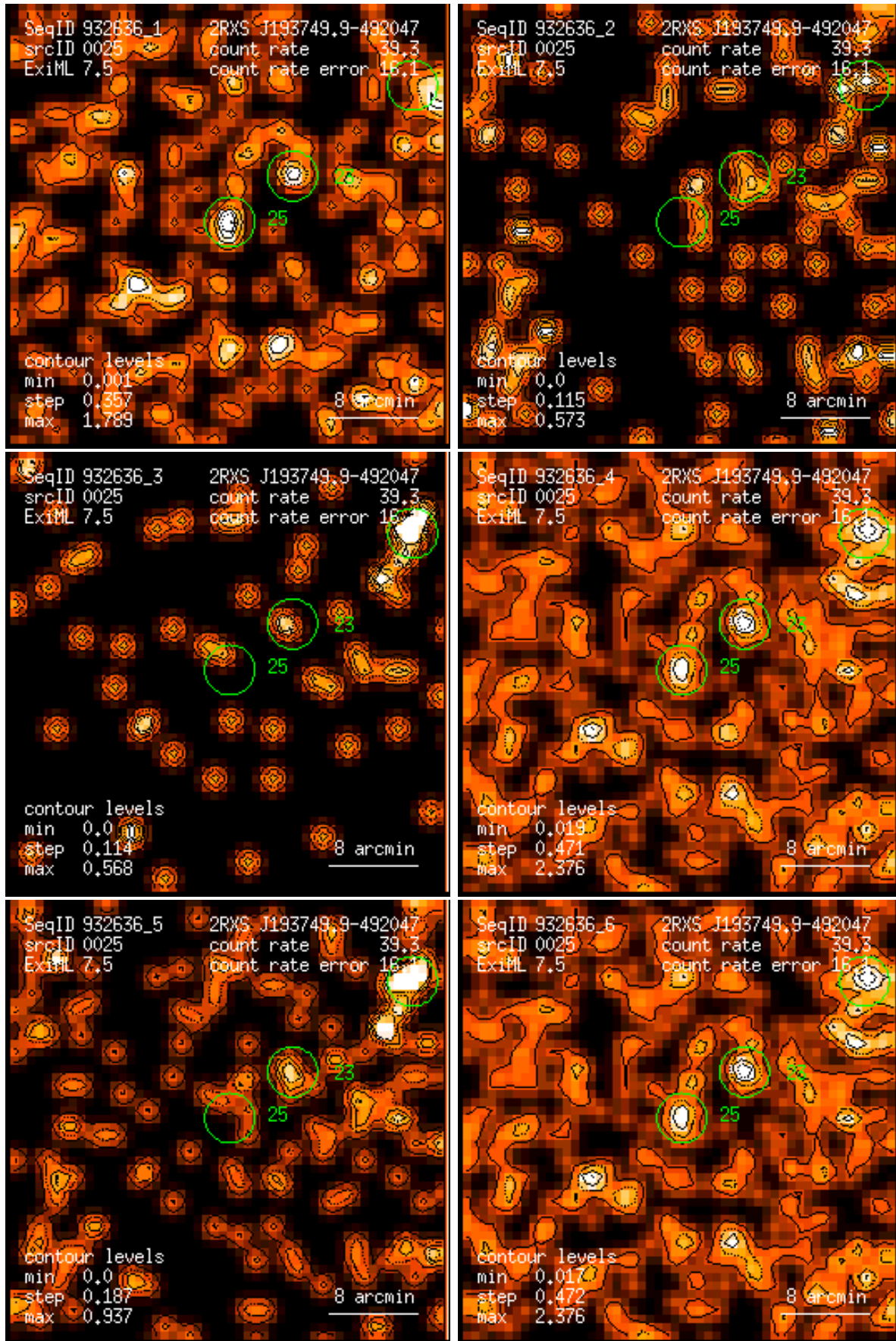
Figure 25: RASS 932636: detection 0025: band rate images, Gaussian filter: (1) PSPC channels 11 – 41, (2) 52 – 90, (3) 91 – 201, (4) 11 – 235, (5) 52 – 201, (6) 11 – 201. Broad band rates in counts/ks. Band rate contour levels in counts/ks/arcmin 2 .
