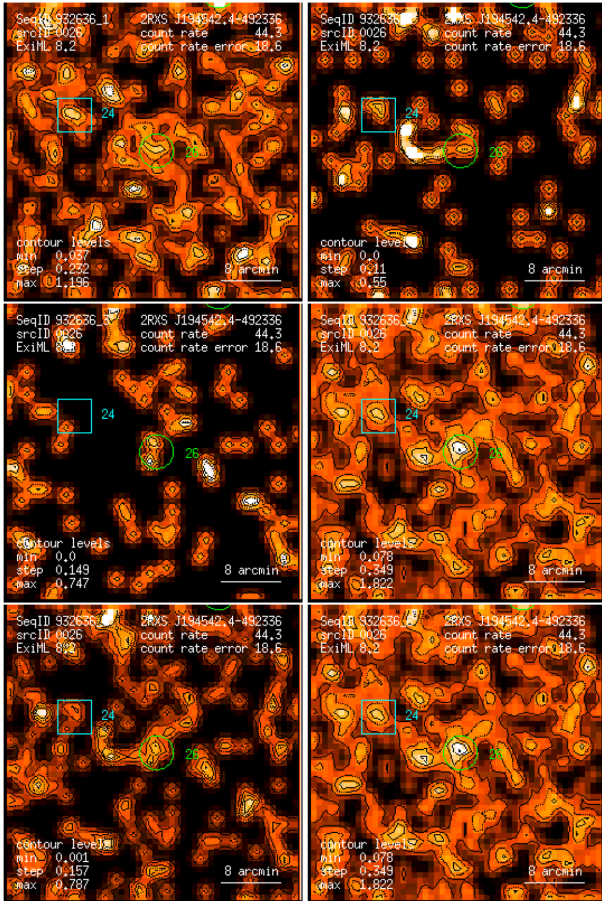
Figure 26: RASS 932636: detection 0026: band rate images, Gaussian filter: (1) PSPC channels 11 – 41, (2) 52 – 90, (3) 91 – 201, (4) 11 – 235, (5) 52 – 201, (6) 11 – 201. Broad band rates in counts/ks. Band rate contour levels in counts/ks/arcmin 2 .
