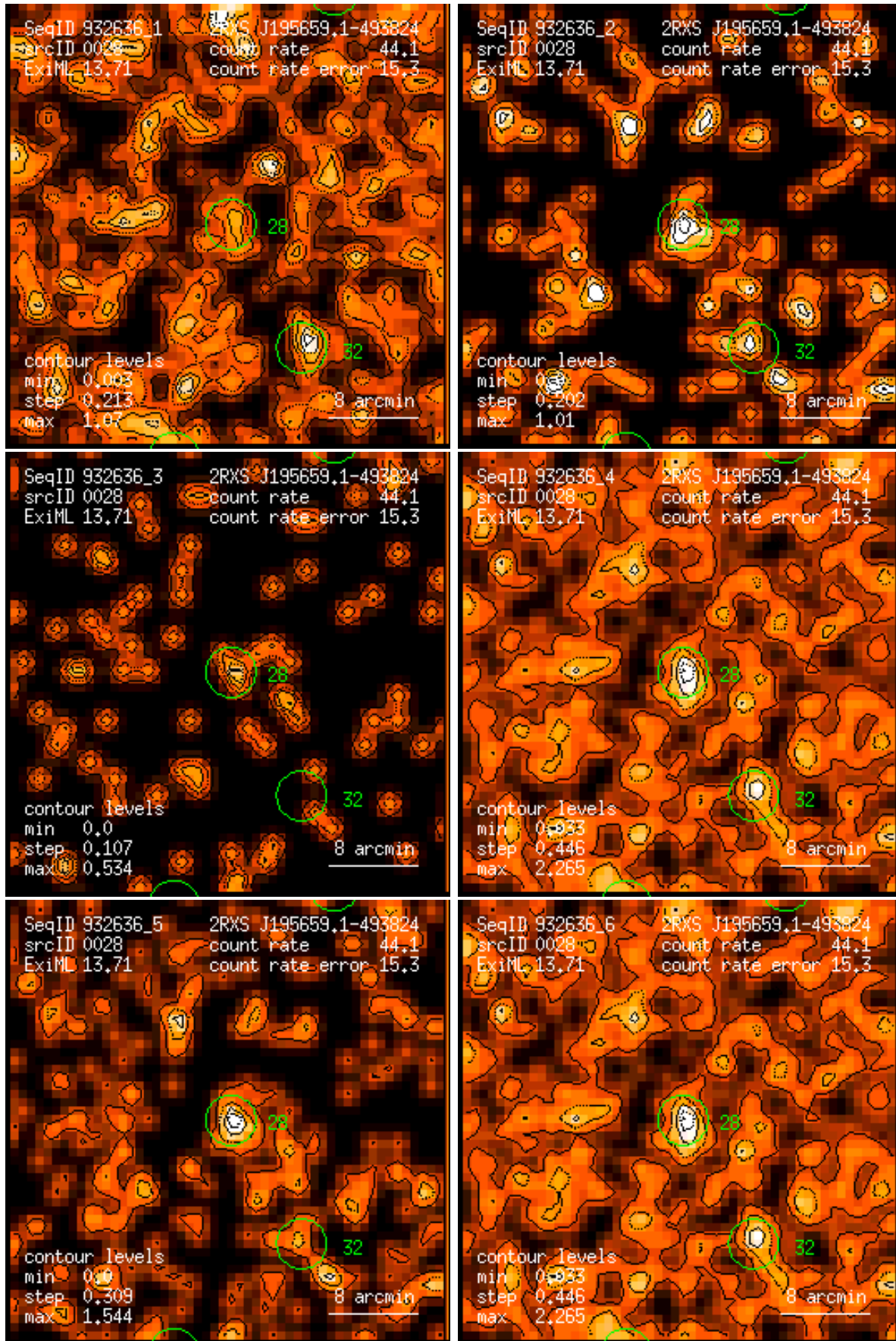
Figure 28: RASS 932636: detection 0028: band rate images, Gaussian filter: (1) PSPC channels 11 – 41, (2) 52 – 90, (3) 91 – 201, (4) 11 – 235, (5) 52 – 201, (6) 11 – 201. Broad band rates in counts/ks. Band rate contour levels in counts/ks/arcmin 2 .
