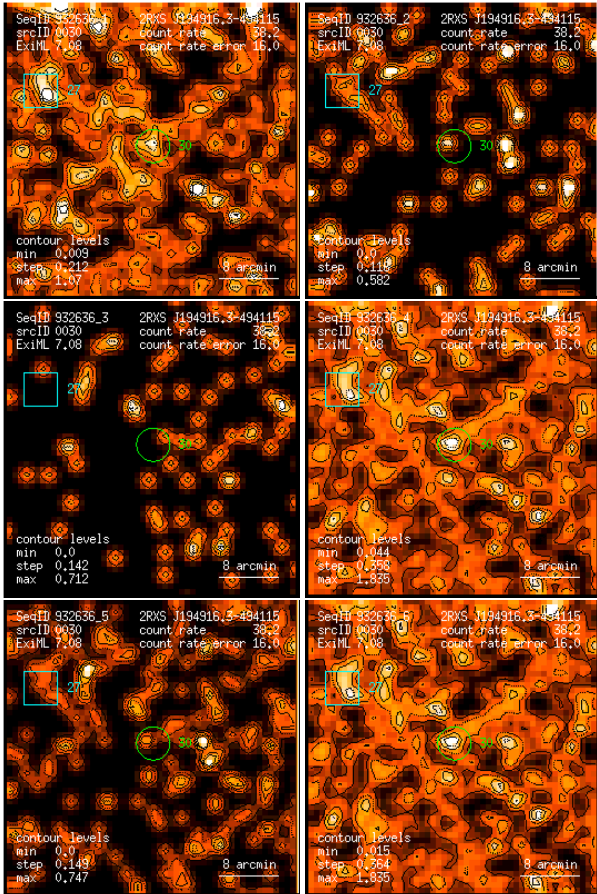
Figure 30: RASS 932636: detection 0030: band rate images, Gaussian filter: (1) PSPC channels 11 – 41, (2) 52 – 90, (3) 91 – 201, (4) 11 – 235, (5) 52 – 201, (6) 11 – 201. Broad band rates in counts/ks. Band rate contour levels in counts/ks/arcmin 2 .
