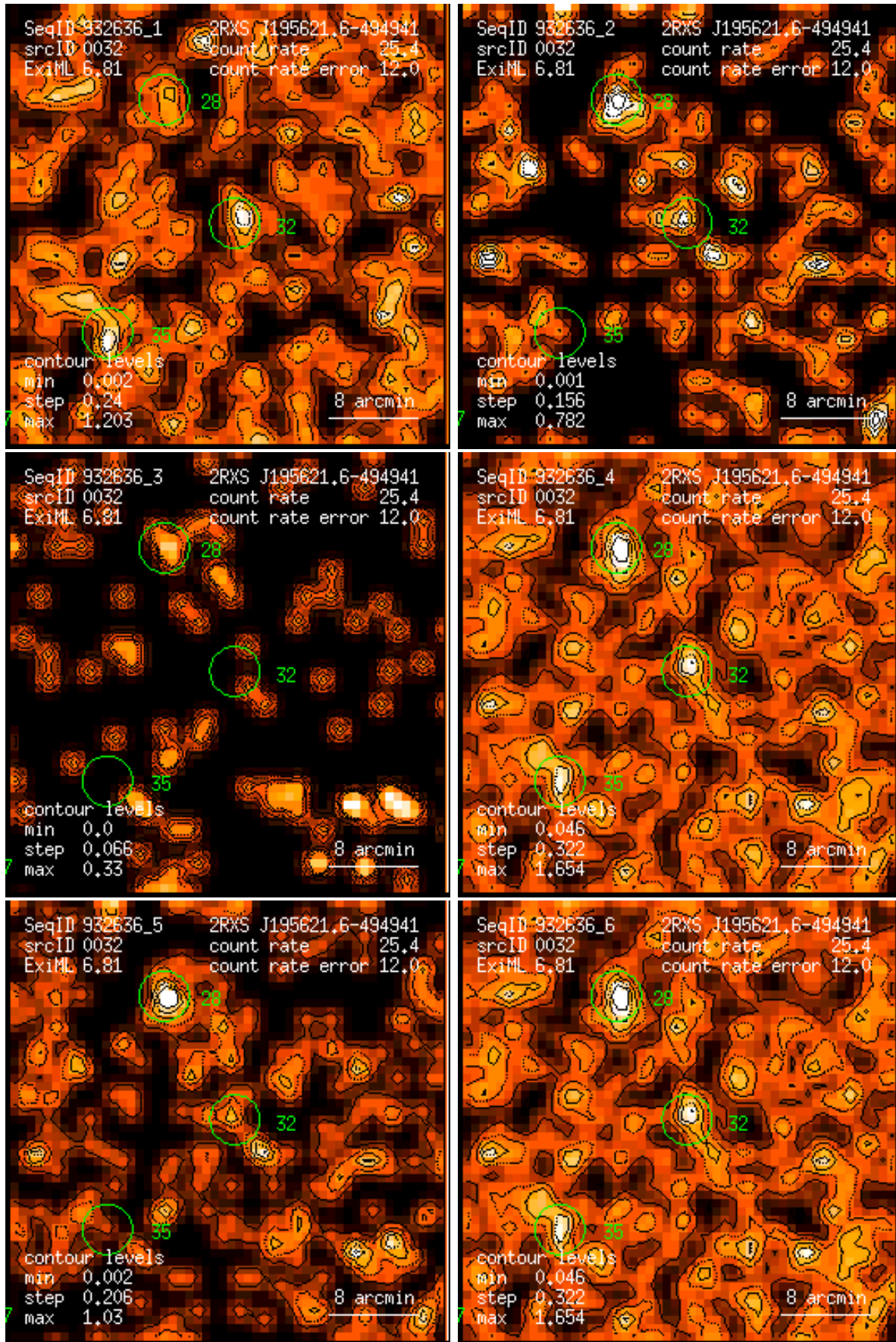
Figure 32: RASS 932636: detection 0032: band rate images, Gaussian filter: (1) PSPC channels 11 – 41, (2) 52 – 90, (3) 91 – 201, (4) 11 – 235, (5) 52 – 201, (6) 11 – 201. Broad band rates in counts/ks. Band rate contour levels in counts/ks/arcmin 2 .
