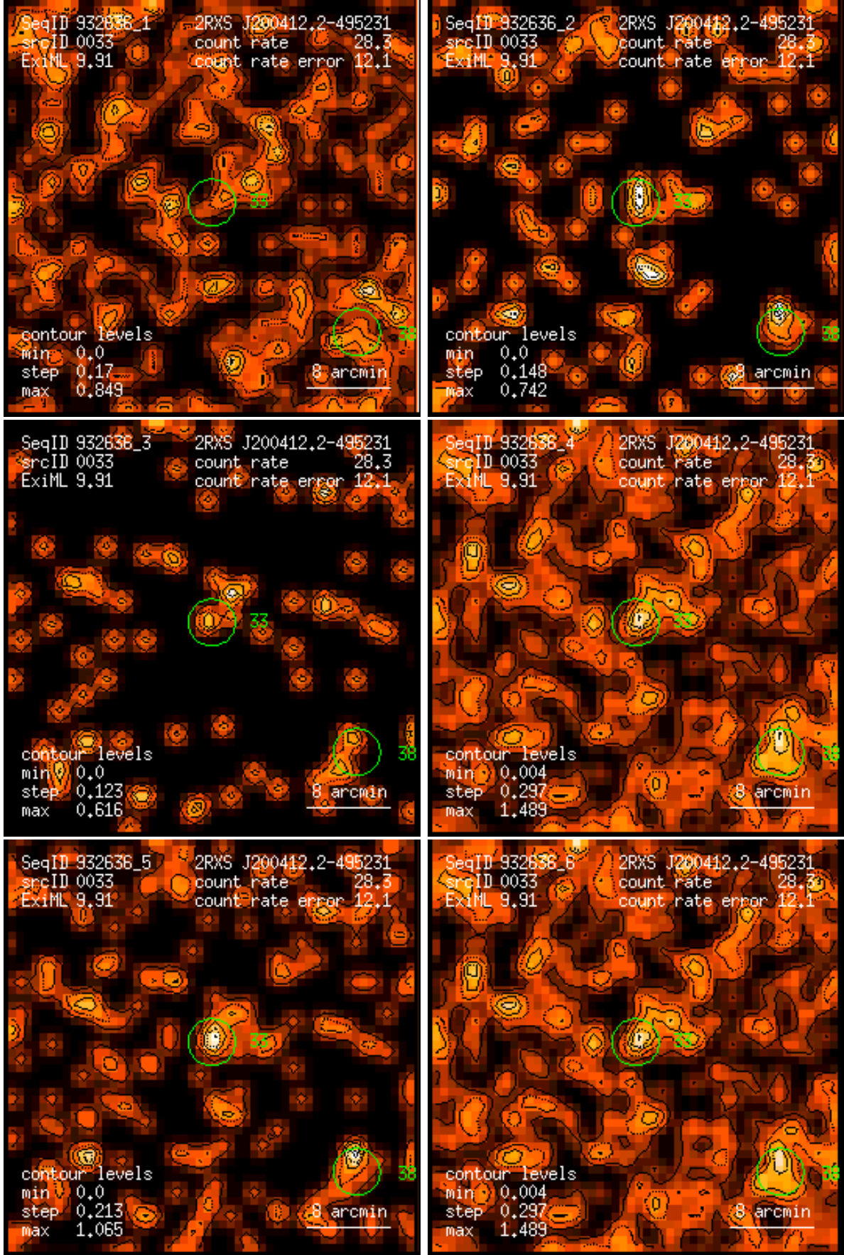
Figure 33: RASS 932636: detection 0033: band rate images, Gaussian filter: (1) PSPC channels 11 – 41, (2) 52 – 90, (3) 91 – 201, (4) 11 – 235, (5) 52 – 201, (6) 11 – 201. Broad band rates in counts/ks. Band rate contour levels in counts/ks/arcmin 2 .
