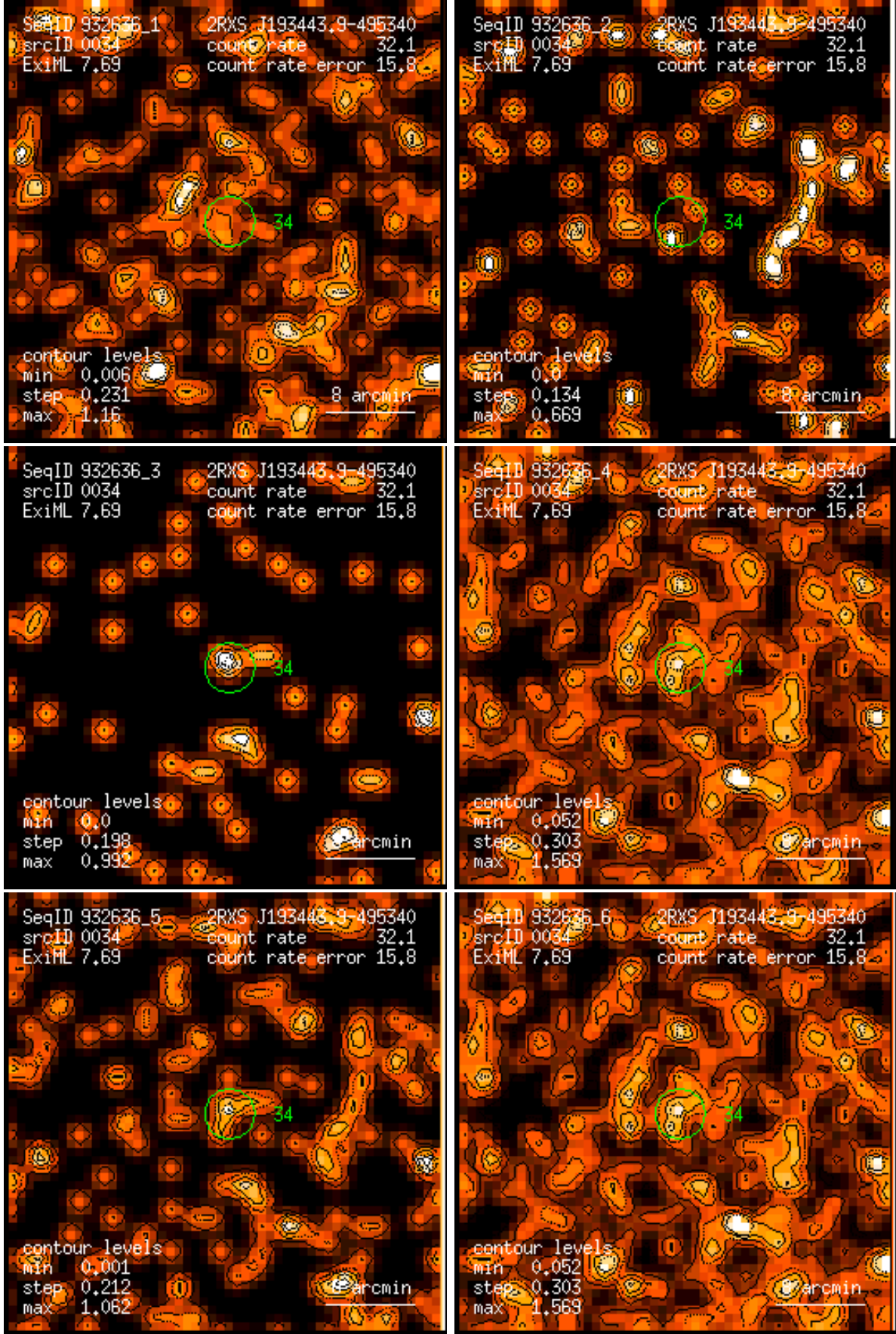
Figure 34: RASS 932636: detection 0034: band rate images, Gaussian filter: (1) PSPC channels 11 – 41, (2) 52 – 90, (3) 91 – 201, (4) 11 – 235, (5) 52 – 201, (6) 11 – 201. Broad band rates in counts/ks. Band rate contour levels in counts/ks/arcmin 2 .
