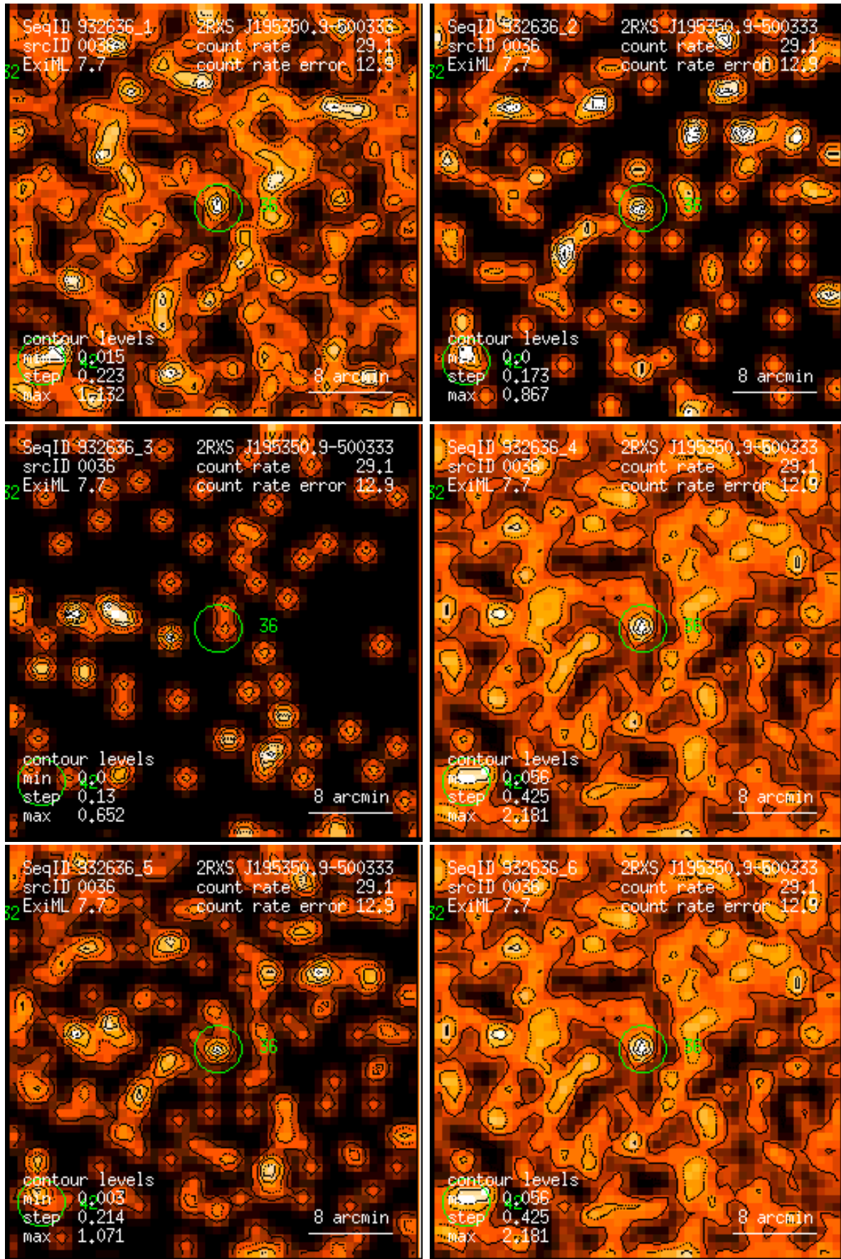
Figure 36: RASS 932636: detection 0036: band rate images, Gaussian filter: (1) PSPC channels 11 – 41, (2) 52 – 90, (3) 91 – 201, (4) 11 – 235, (5) 52 – 201, (6) 11 – 201. Broad band rates in counts/ks. Band rate contour levels in counts/ks/arcmin 2 .
