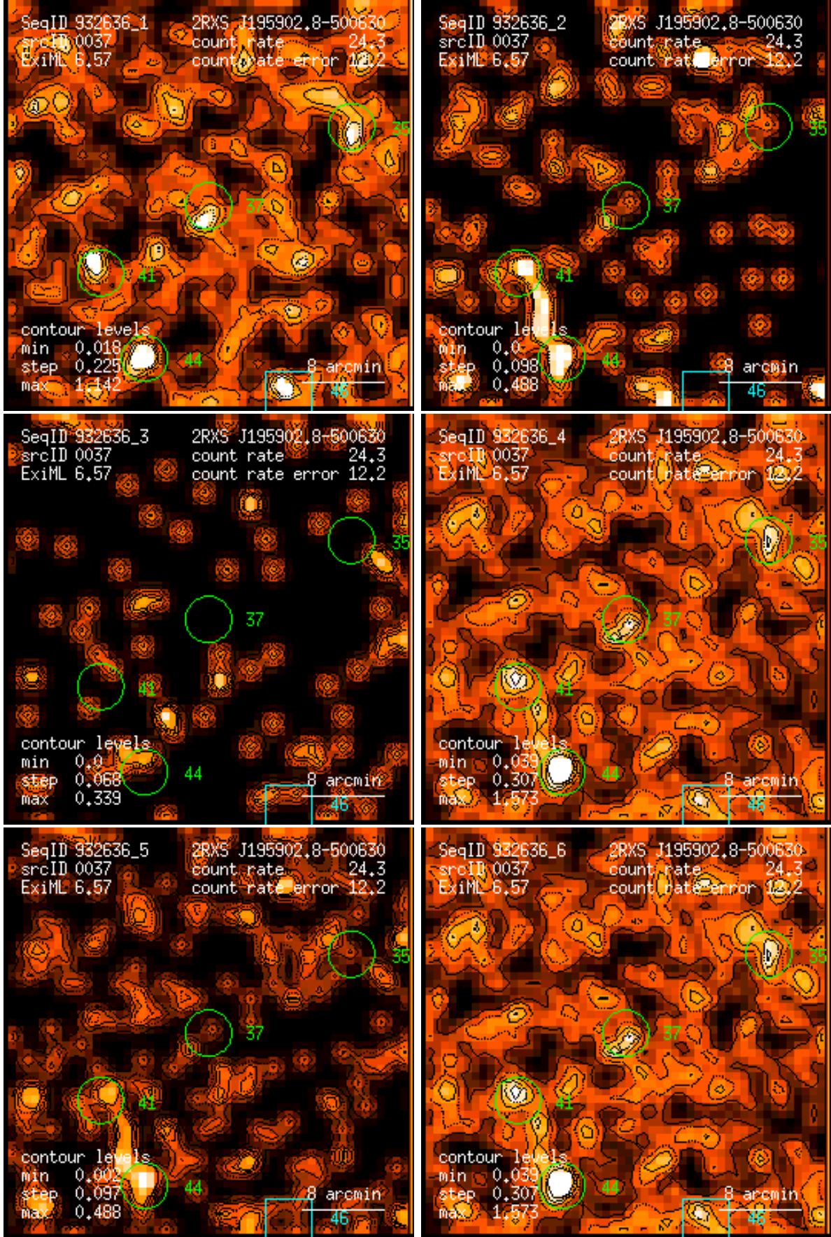
Figure 37: RASS 932636: detection 0037: band rate images, Gaussian filter: (1) PSPC channels 11 – 41, (2) 52 – 90, (3) 91 – 201, (4) 11 – 235, (5) 52 – 201, (6) 11 – 201. Broad band rates in counts/ks. Band rate contour levels in counts/ks/arcmin 2 .
