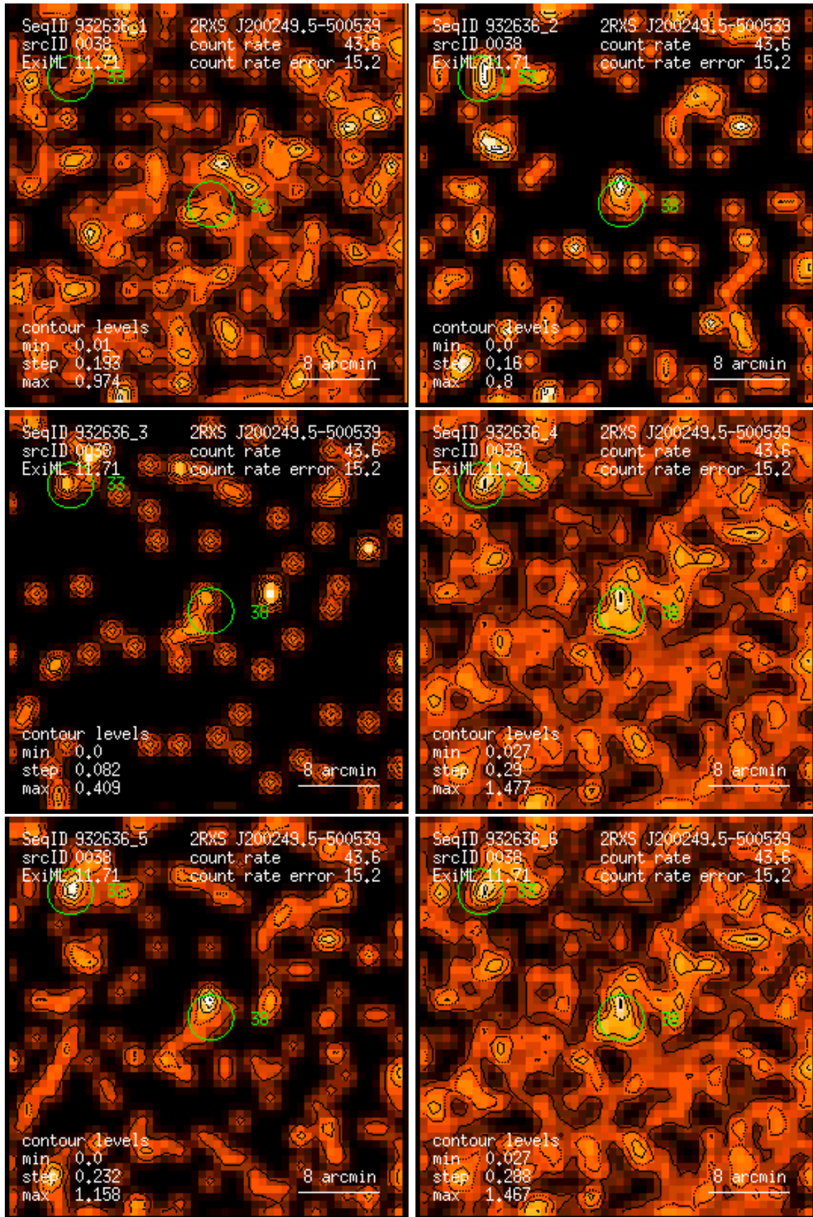
Figure 38: RASS 932636: detection 0038: band rate images, Gaussian filter: (1) PSPC channels 11 – 41, (2) 52 – 90, (3) 91 – 201, (4) 11 – 235, (5) 52 – 201, (6) 11 – 201. Broad band rates in counts/ks. Band rate contour levels in counts/ks/arcmin 2 .
