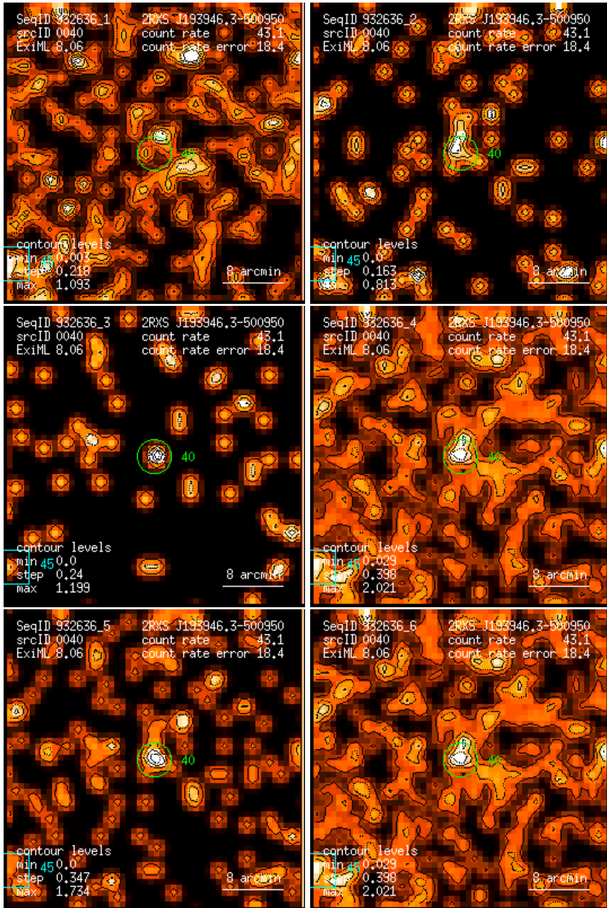
Figure 40: RASS 932636: detection 0040: band rate images, Gaussian filter: (1) PSPC channels 11 – 41, (2) 52 – 90, (3) 91 – 201, (4) 11 – 235, (5) 52 – 201, (6) 11 – 201. Broad band rates in counts/ks. Band rate contour levels in counts/ks/arcmin 2 .
