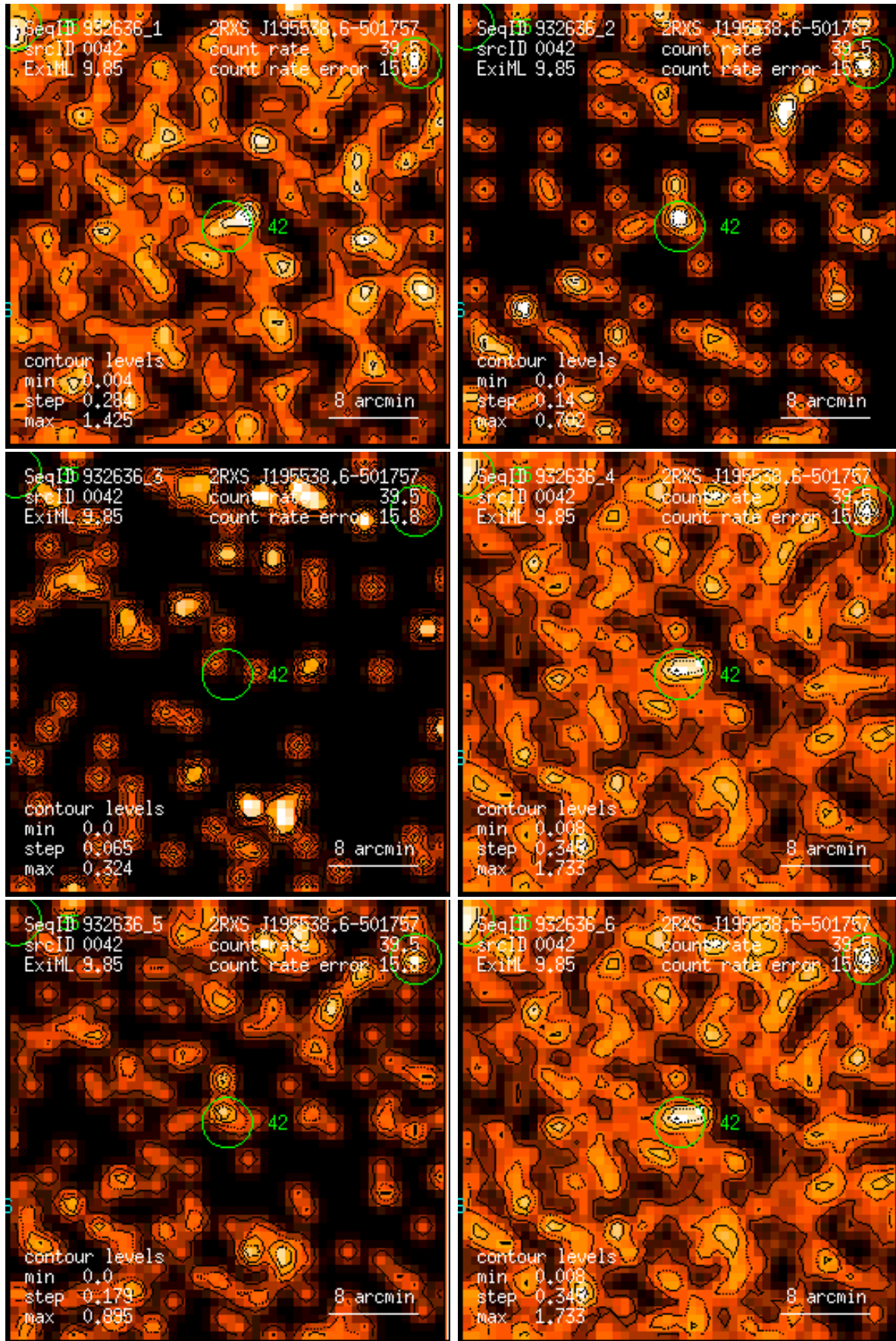
Figure 42: RASS 932636: detection 0042: band rate images, Gaussian filter: (1) PSPC channels 11 – 41, (2) 52 – 90, (3) 91 – 201, (4) 11 – 235, (5) 52 – 201, (6) 11 – 201. Broad band rates in counts/ks. Band rate contour levels in counts/ks/arcmin 2 .
