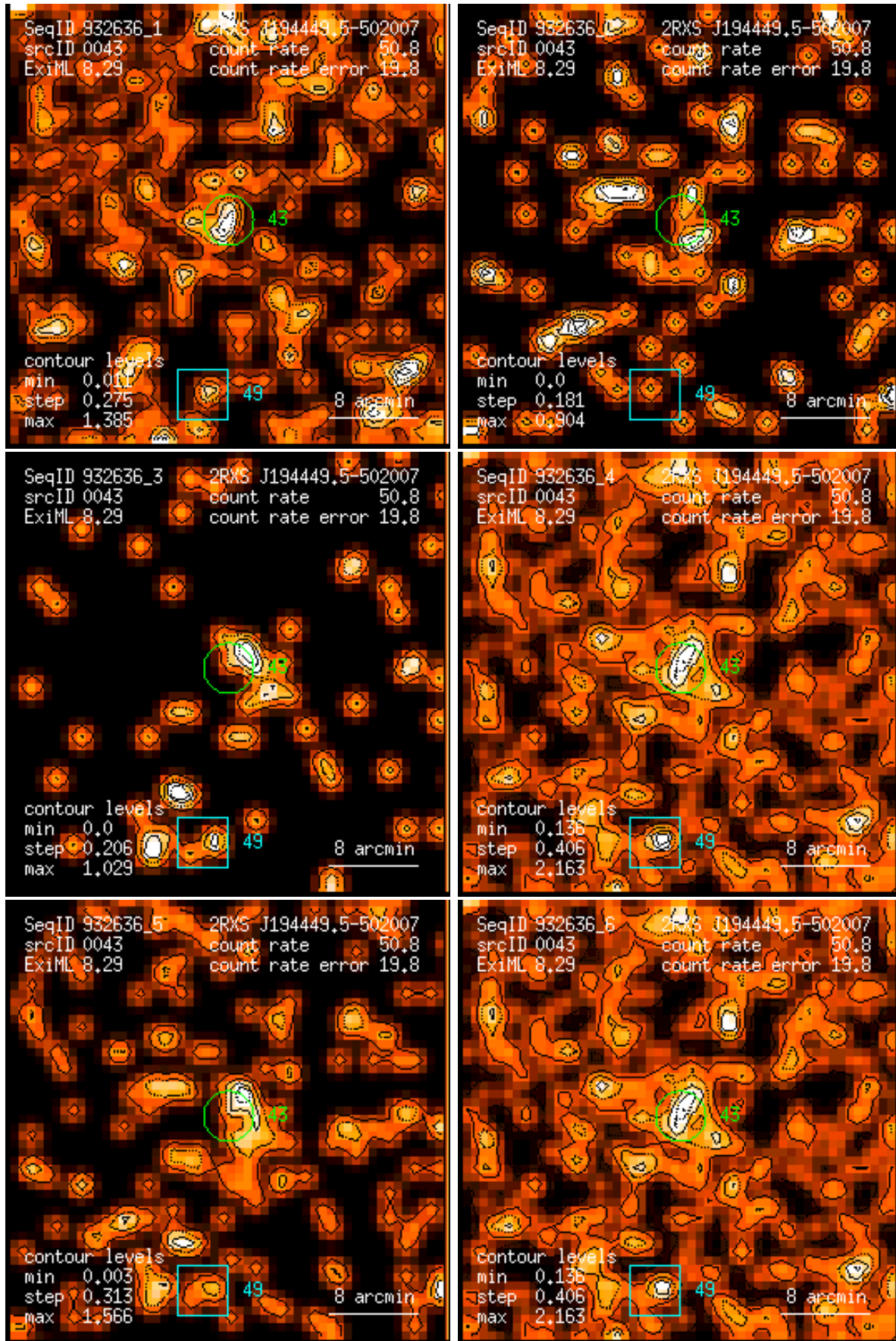
Figure 43: RASS 932636: detection 0043: band rate images, Gaussian filter: (1) PSPC channels 11 – 41, (2) 52 – 90, (3) 91 – 201, (4) 11 – 235, (5) 52 – 201, (6) 11 – 201. Broad band rates in counts/ks. Band rate contour levels in counts/ks/arcmin 2 .
