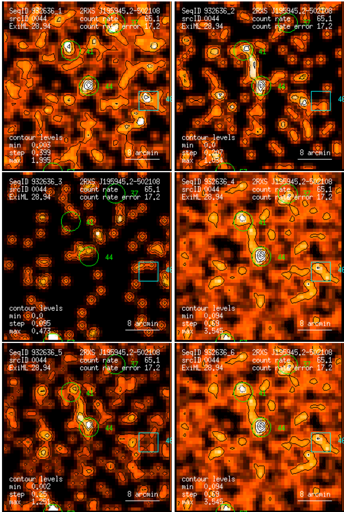
Figure 44: RASS 932636: detection 0044: band rate images, Gaussian filter: (1) PSPC channels 11 – 41, (2) 52 – 90, (3) 91 – 201, (4) 11 – 235, (5) 52 – 201, (6) 11 – 201. Broad band rates in counts/ks. Band rate contour levels in counts/ks/arcmin 2 .
