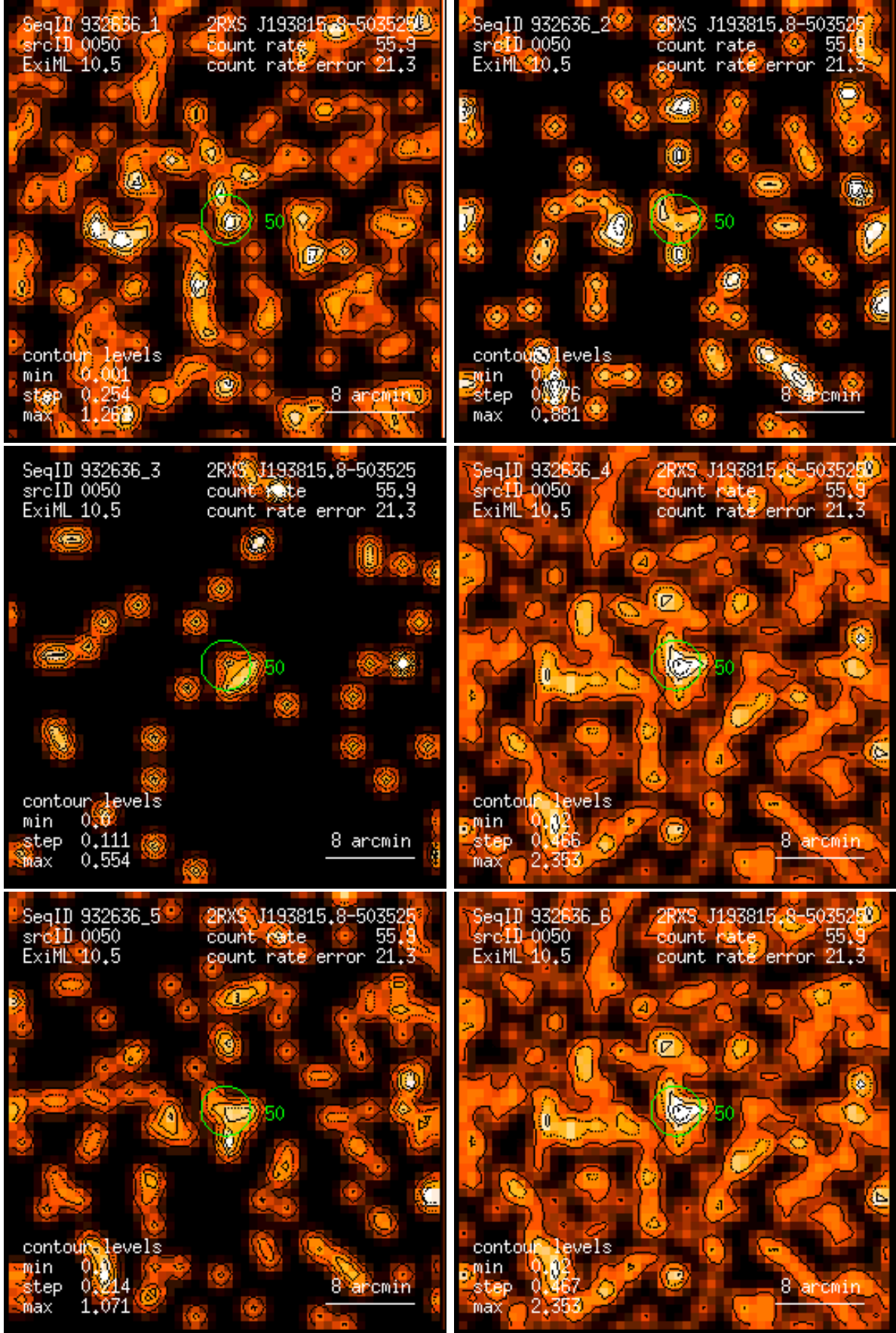
Figure 50: RASS 932636: detection 0050: band rate images, Gaussian filter: (1) PSPC channels 11 – 41, (2) 52 – 90, (3) 91 – 201, (4) 11 – 235, (5) 52 – 201, (6) 11 – 201. Broad band rates in counts/ks. Band rate contour levels in counts/ks/arcmin 2 .
