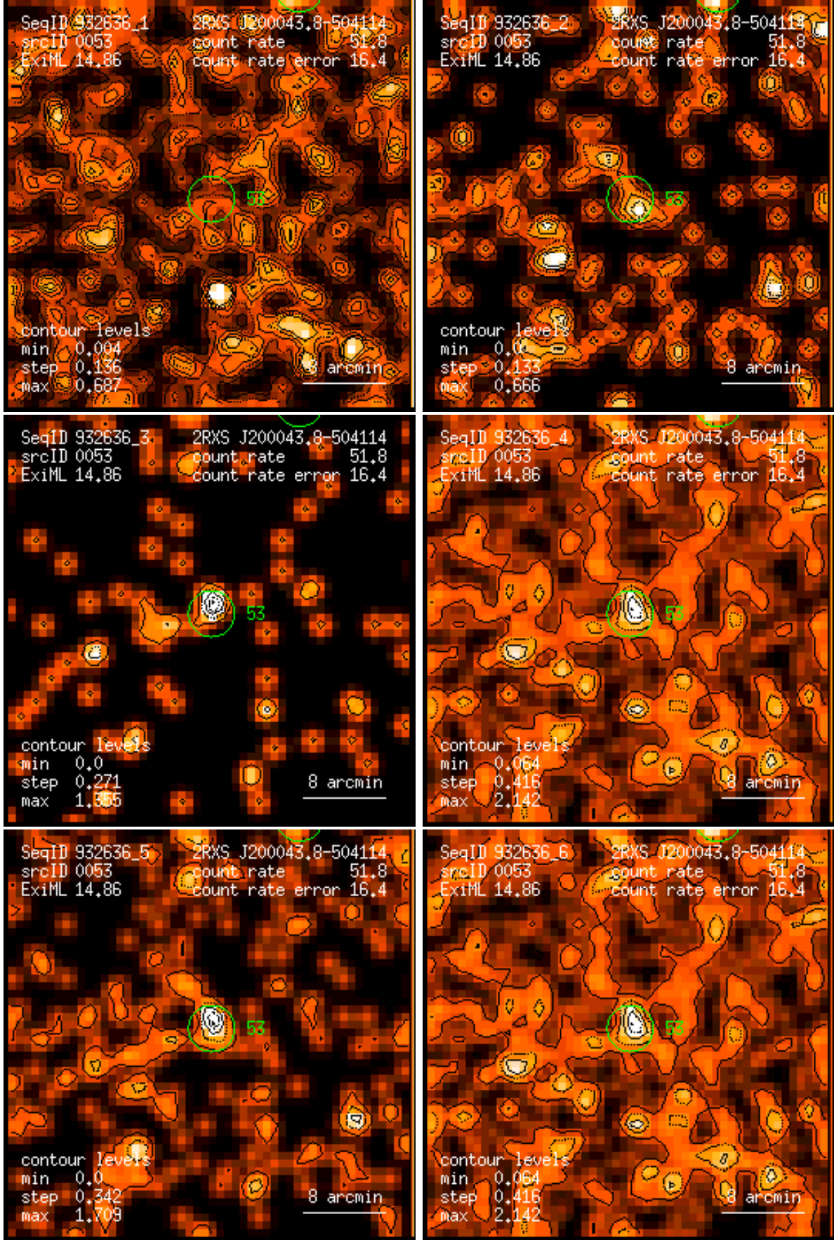
Figure 53: RASS 932636: detection 0053: band rate images, Gaussian filter: (1) PSPC channels 11 – 41, (2) 52 – 90, (3) 91 – 201, (4) 11 – 235, (5) 52 – 201, (6) 11 – 201. Broad band rates in counts/ks. Band rate contour levels in counts/ks/arcmin 2 .
