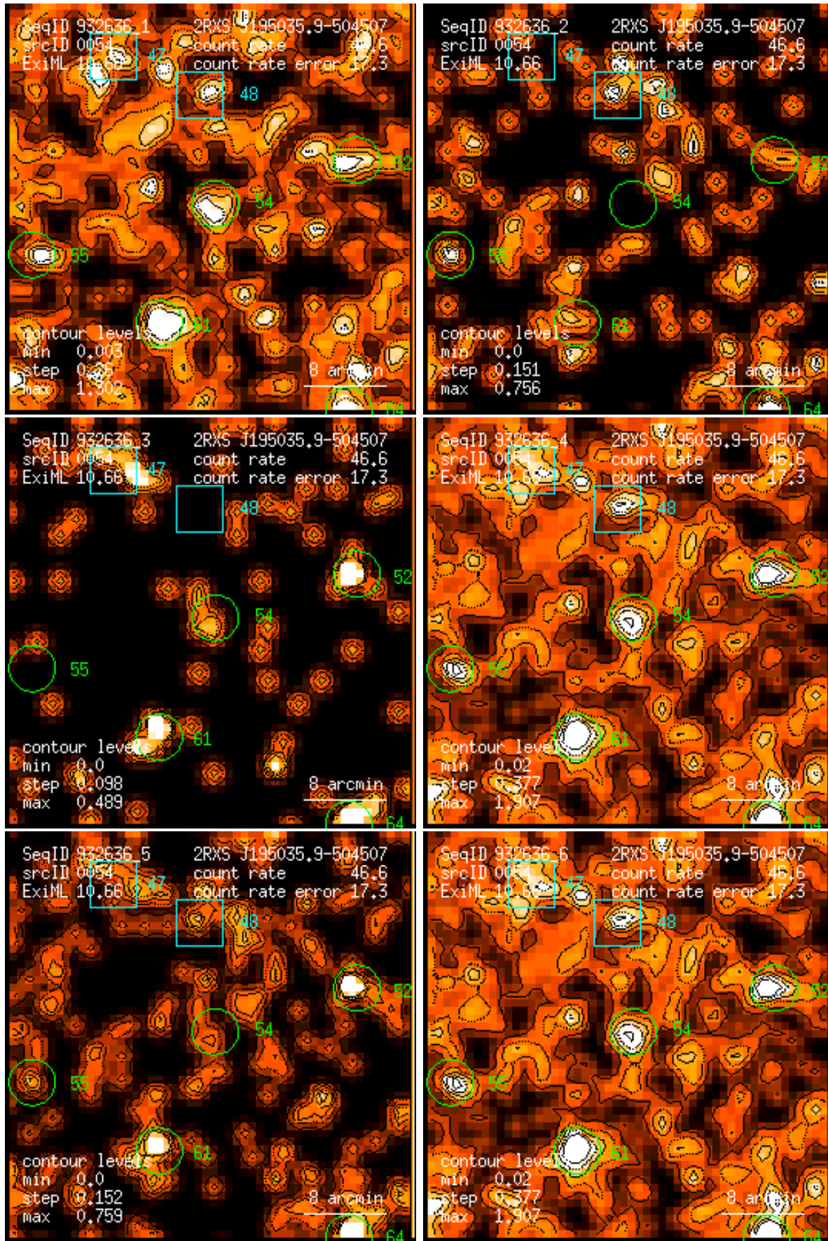
Figure 54: RASS 932636: detection 0054: band rate images, Gaussian filter: (1) PSPC channels 11 – 41, (2) 52 – 90, (3) 91 – 201, (4) 11 – 235, (5) 52 – 201, (6) 11 – 201. Broad band rates in counts/ks. Band rate contour levels in counts/ks/arcmin 2 .
