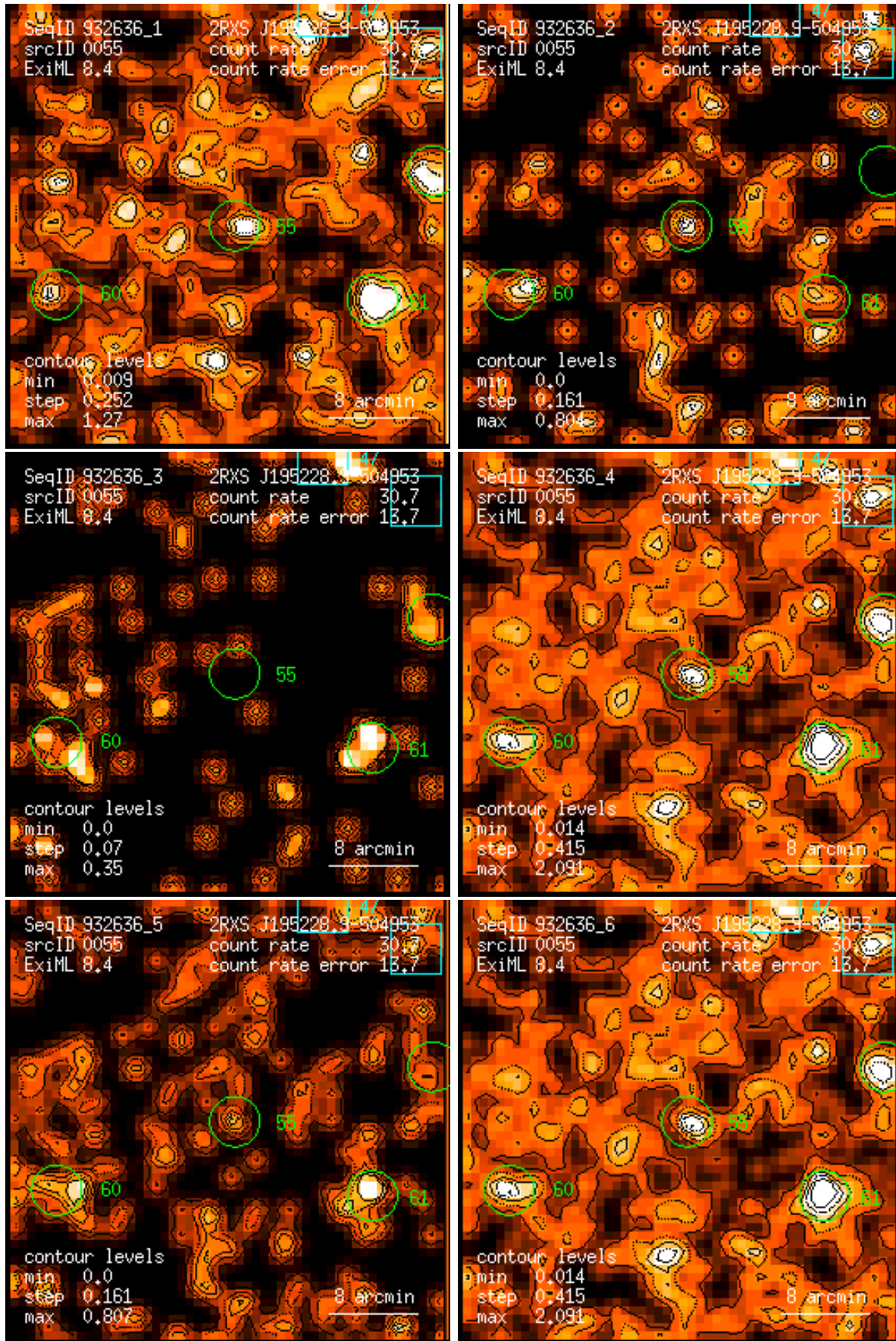
Figure 55: RASS 932636: detection 0055: band rate images, Gaussian filter: (1) PSPC channels 11 – 41, (2) 52 – 90, (3) 91 – 201, (4) 11 – 235, (5) 52 – 201, (6) 11 – 201. Broad band rates in counts/ks. Band rate contour levels in counts/ks/arcmin 2 .
