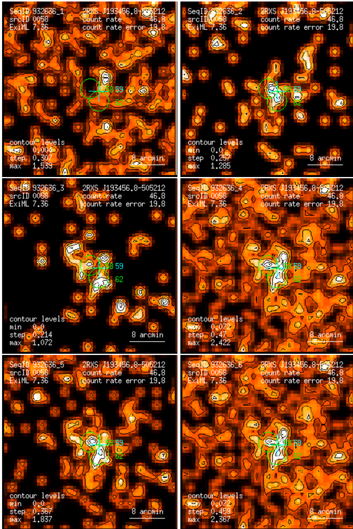
Figure 58: RASS 932636: detection 0058: band rate images, Gaussian filter: (1) PSPC channels 11 – 41, (2) 52 – 90, (3) 91 – 201, (4) 11 – 235, (5) 52 – 201, (6) 11 – 201. Broad band rates in counts/ks. Band rate contour levels in counts/ks/arcmin 2 .
