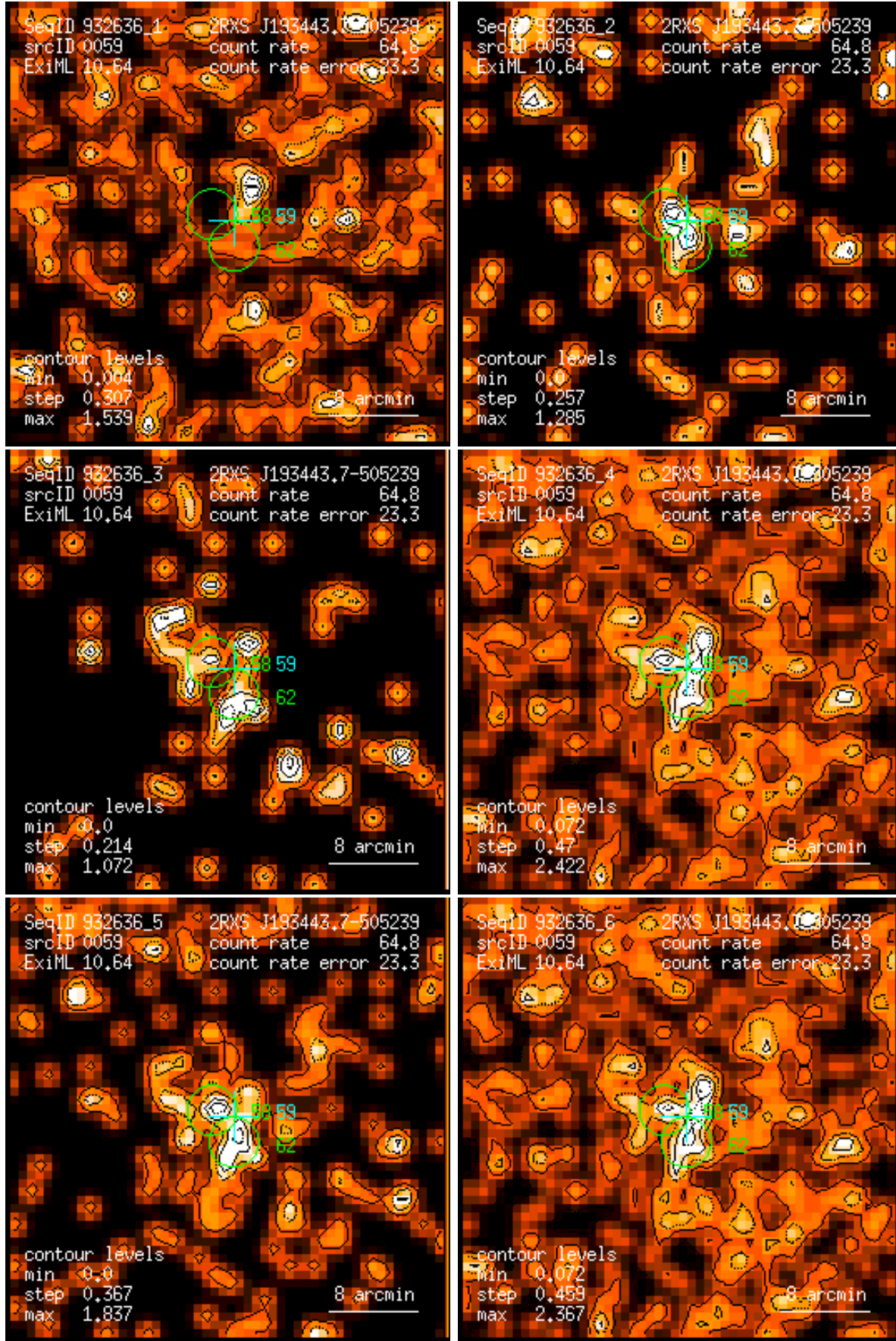
Figure 59: RASS 932636: detection 0059: band rate images, Gaussian filter: (1) PSPC channels 11 – 41, (2) 52 – 90, (3) 91 – 201, (4) 11 – 235, (5) 52 – 201, (6) 11 – 201. Broad band rates in counts/ks. Band rate contour levels in counts/ks/arcmin 2 .
