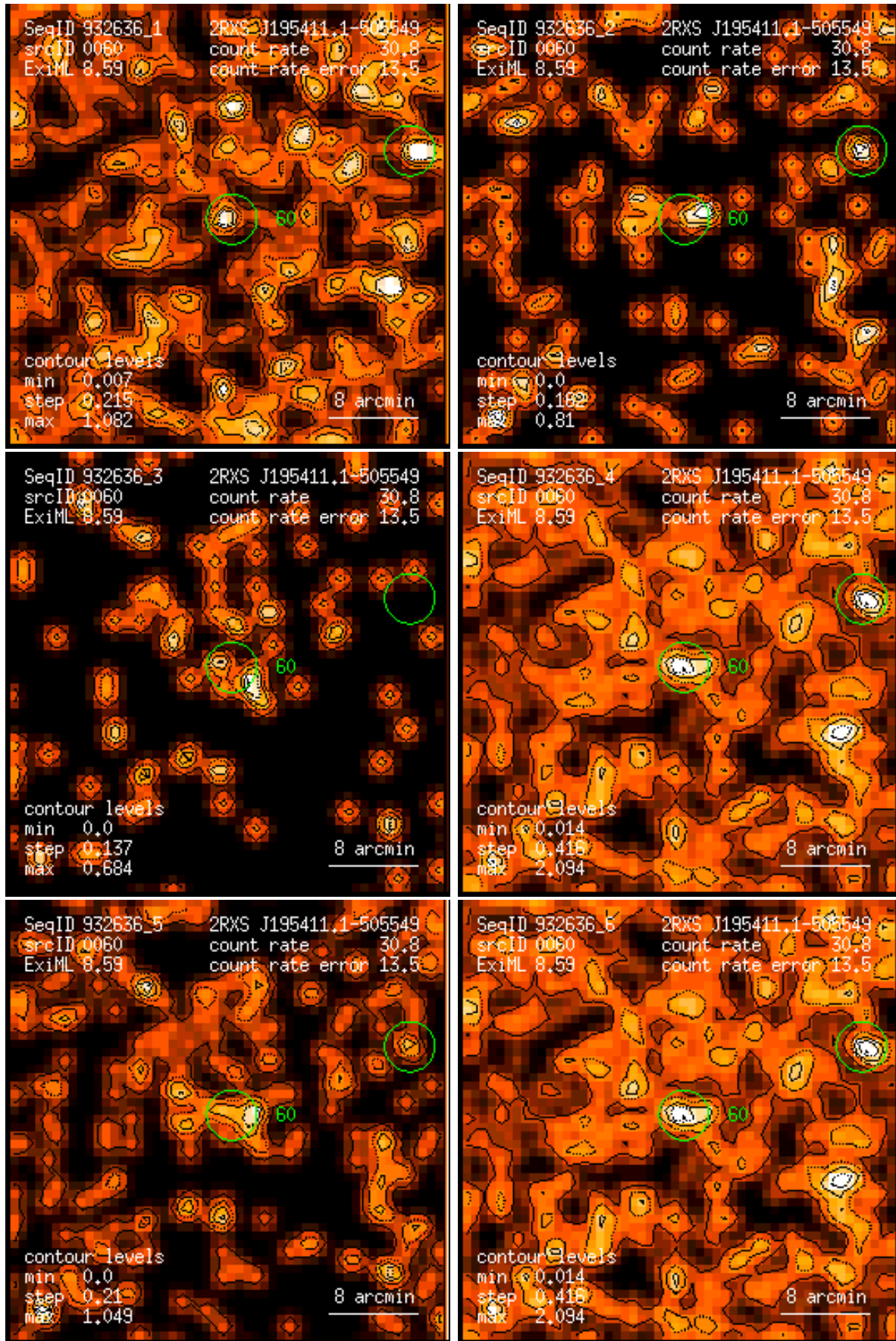
Figure 60: RASS 932636: detection 0060: band rate images, Gaussian filter: (1) PSPC channels 11 – 41, (2) 52 – 90, (3) 91 – 201, (4) 11 – 235, (5) 52 – 201, (6) 11 – 201. Broad band rates in counts/ks. Band rate contour levels in counts/ks/arcmin 2 .
