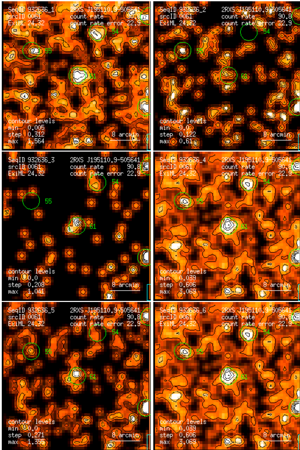
Figure 61: RASS 932636: detection 0061: band rate images, Gaussian filter: (1) PSPC channels 11 – 41, (2) 52 – 90, (3) 91 – 201, (4) 11 – 235, (5) 52 – 201, (6) 11 – 201. Broad band rates in counts/ks. Band rate contour levels in counts/ks/arcmin 2 .
