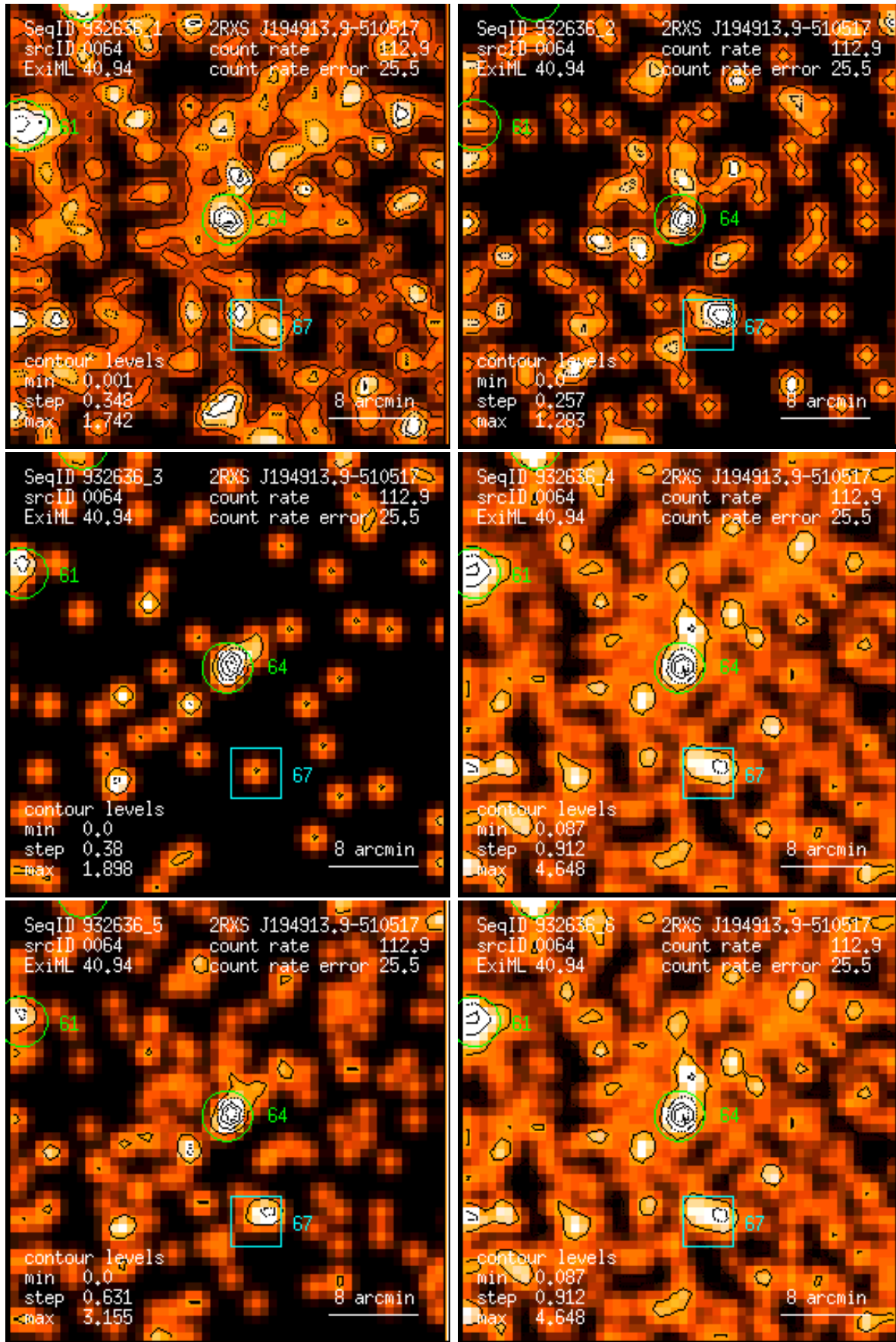
Figure 64: RASS 932636: detection 0064: band rate images, Gaussian filter: (1) PSPC channels 11 – 41, (2) 52 – 90, (3) 91 – 201, (4) 11 – 235, (5) 52 – 201, (6) 11 – 201. Broad band rates in counts/ks. Band rate contour levels in counts/ks/arcmin 2 .
