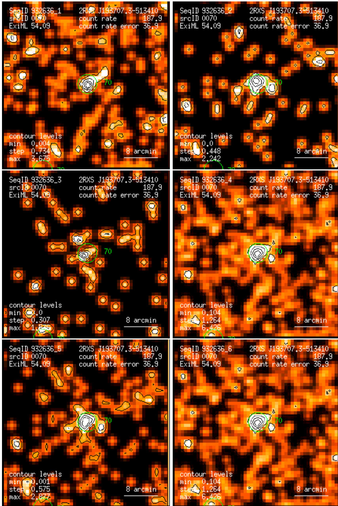
Figure 70: RASS 932636: detection 0070: band rate images, Gaussian filter: (1) PSPC channels 11 – 41, (2) 52 – 90, (3) 91 – 201, (4) 11 – 235, (5) 52 – 201, (6) 11 – 201. Broad band rates in counts/ks. Band rate contour levels in counts/ks/arcmin 2 .
