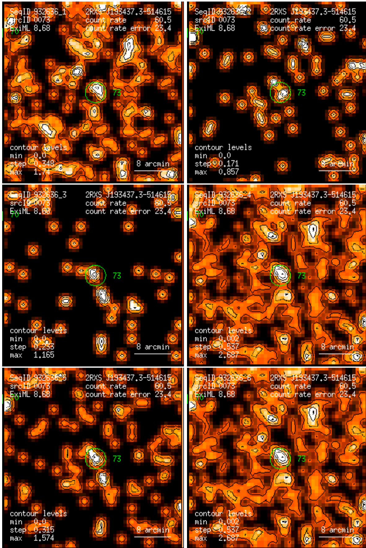
Figure 73: RASS 932636: detection 0073: band rate images, Gaussian filter: (1) PSPC channels 11 – 41, (2) 52 – 90, (3) 91 – 201, (4) 11 – 235, (5) 52 – 201, (6) 11 – 201. Broad band rates in counts/ks. Band rate contour levels in counts/ks/arcmin 2 .
