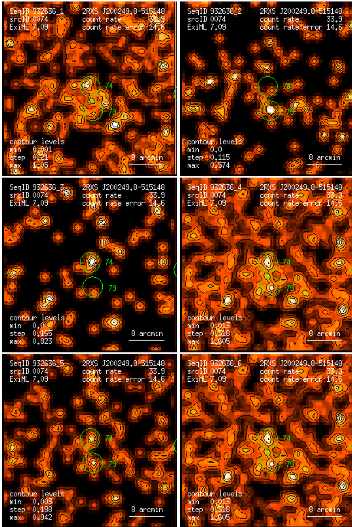
Figure 74: RASS 932636: detection 0074: band rate images, Gaussian filter: (1) PSPC channels 11 – 41, (2) 52 – 90, (3) 91 – 201, (4) 11 – 235, (5) 52 – 201, (6) 11 – 201. Broad band rates in counts/ks. Band rate contour levels in counts/ks/arcmin 2 .
