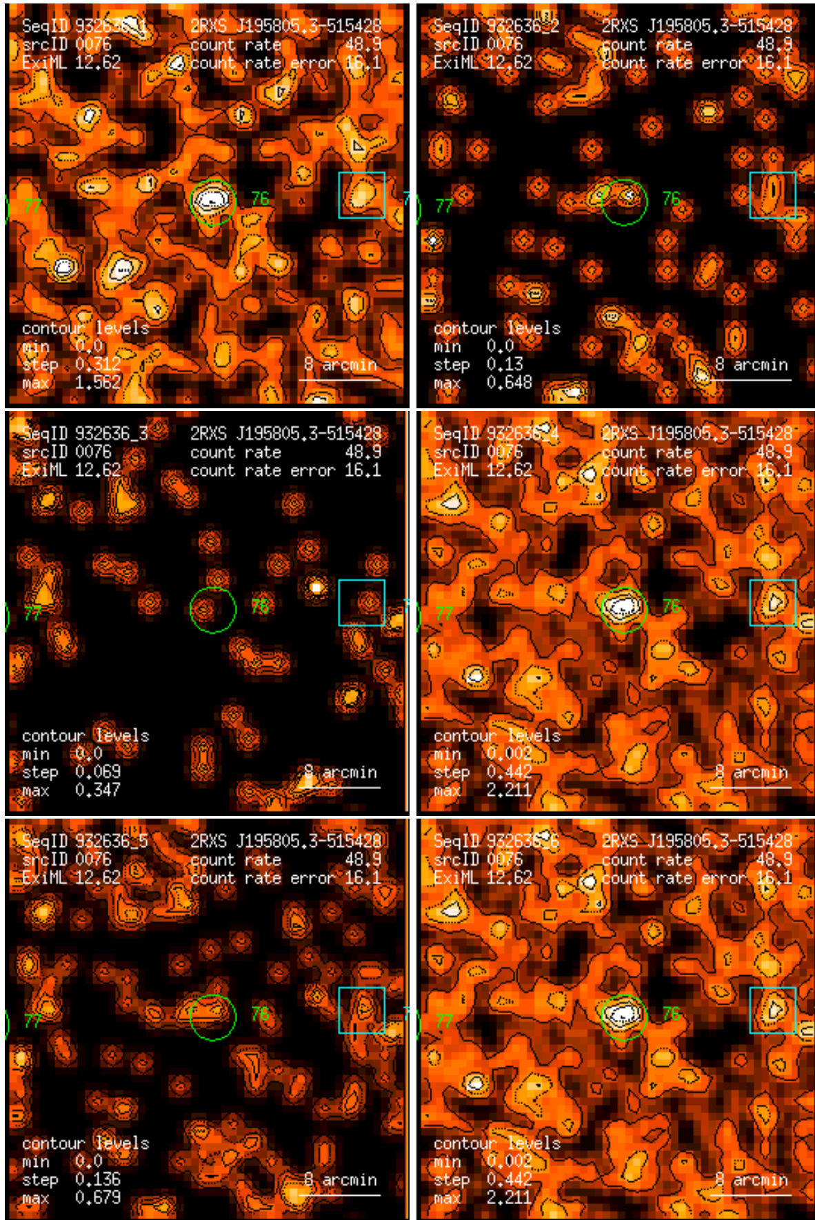
Figure 76: RASS 932636: detection 0076: band rate images, Gaussian filter: (1) PSPC channels 11 – 41, (2) 52 – 90, (3) 91 – 201, (4) 11 – 235, (5) 52 – 201, (6) 11 – 201. Broad band rates in counts/ks. Band rate contour levels in counts/ks/arcmin 2 .
