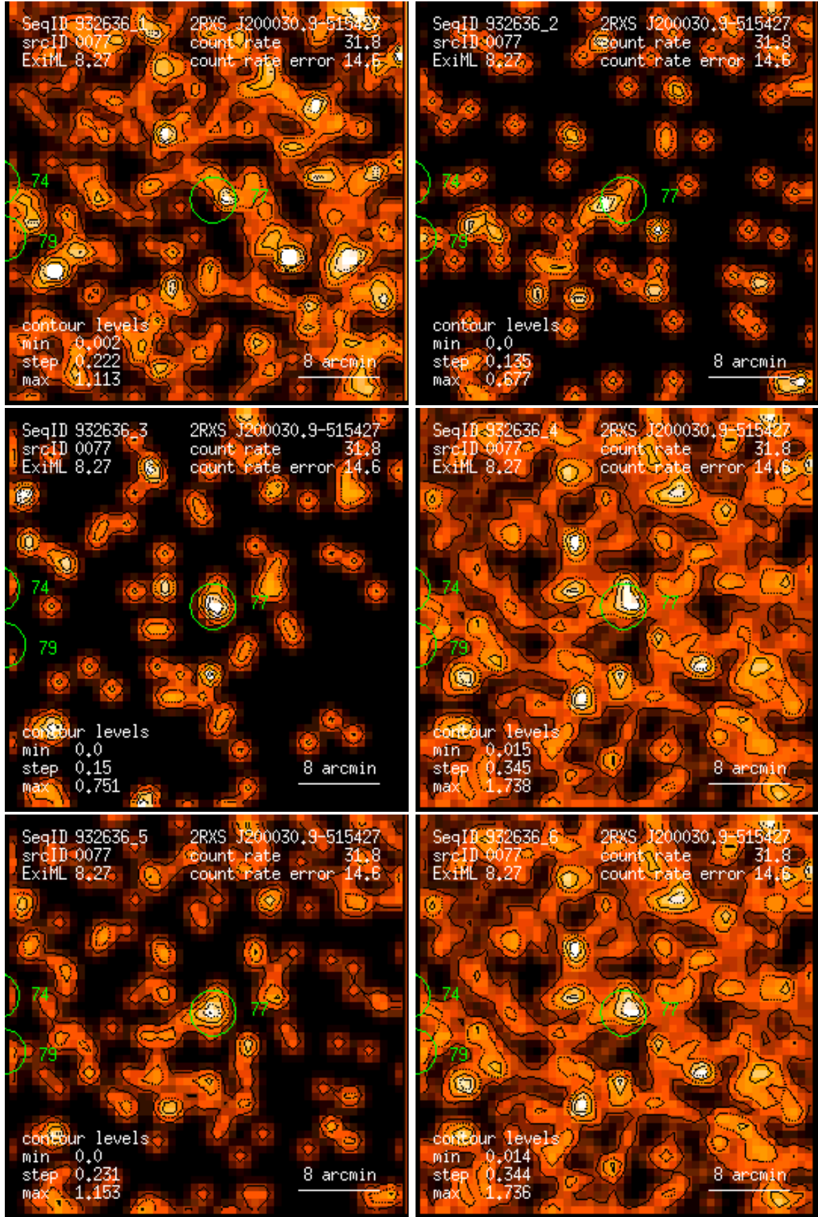
Figure 77: RASS 932636: detection 0077: band rate images, Gaussian filter: (1) PSPC channels 11 – 41, (2) 52 – 90, (3) 91 – 201, (4) 11 – 235, (5) 52 – 201, (6) 11 – 201. Broad band rates in counts/ks. Band rate contour levels in counts/ks/arcmin 2 .
