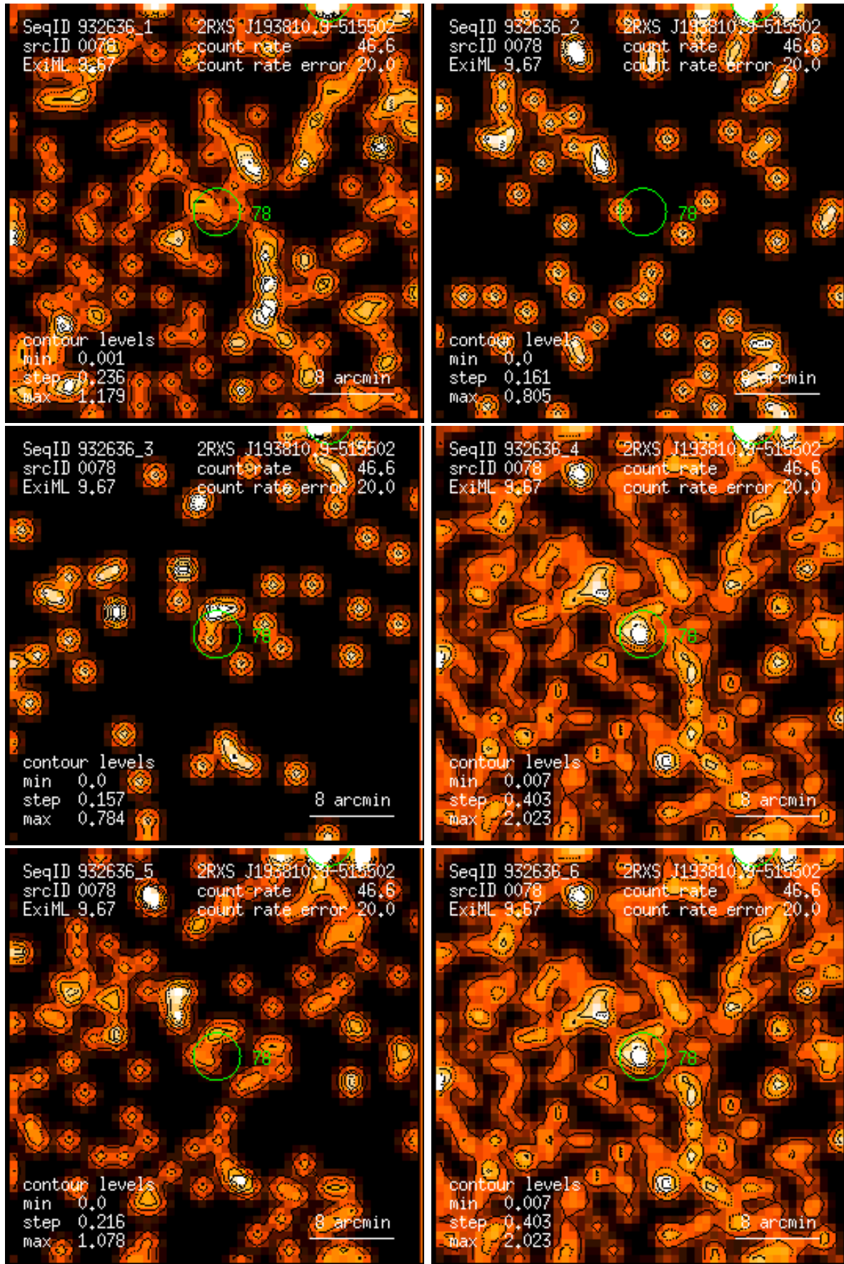
Figure 78: RASS 932636: detection 0078: band rate images, Gaussian filter: (1) PSPC channels 11 – 41, (2) 52 – 90, (3) 91 – 201, (4) 11 – 235, (5) 52 – 201, (6) 11 – 201. Broad band rates in counts/ks. Band rate contour levels in counts/ks/arcmin 2 .
