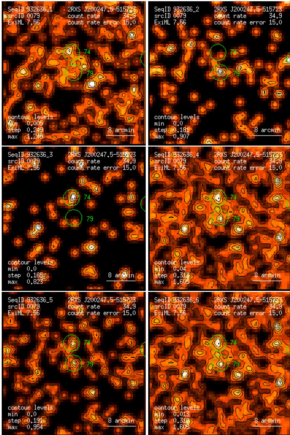
Figure 79: RASS 932636: detection 0079: band rate images, Gaussian filter: (1) PSPC channels 11 – 41, (2) 52 – 90, (3) 91 – 201, (4) 11 – 235, (5) 52 – 201, (6) 11 – 201. Broad band rates in counts/ks. Band rate contour levels in counts/ks/arcmin 2 .
